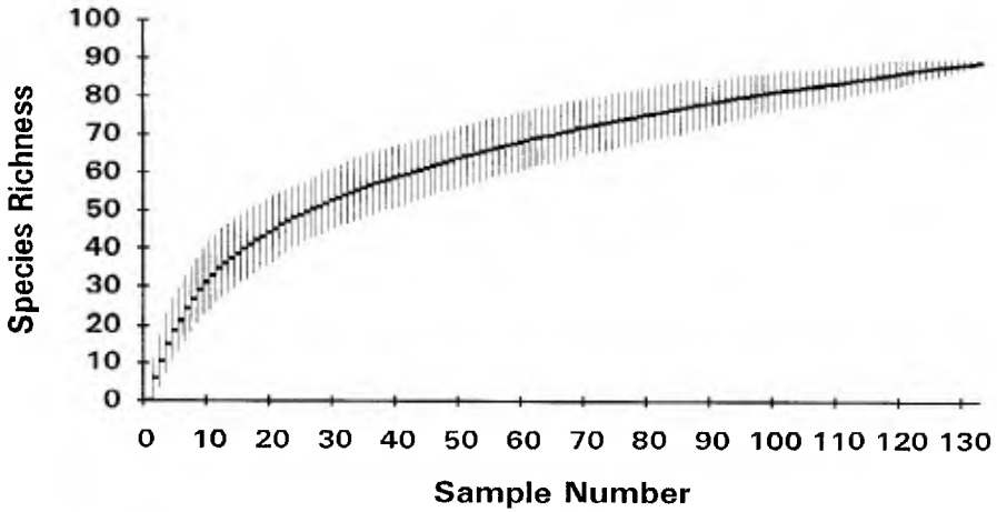
Figure 2.—The empirical species accumulation curve for the data of Appendix. Samples were accumulated randomly 100 times, and the mean \pm two standard deviations plotted.
