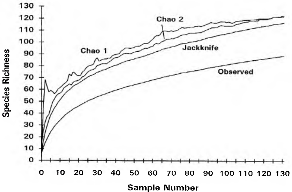
Figure 3.—Mean values of observed species richness and Chao 1, Chao 2, and jackknife estimators at each sample increment for 100 random orders of sample addition.
