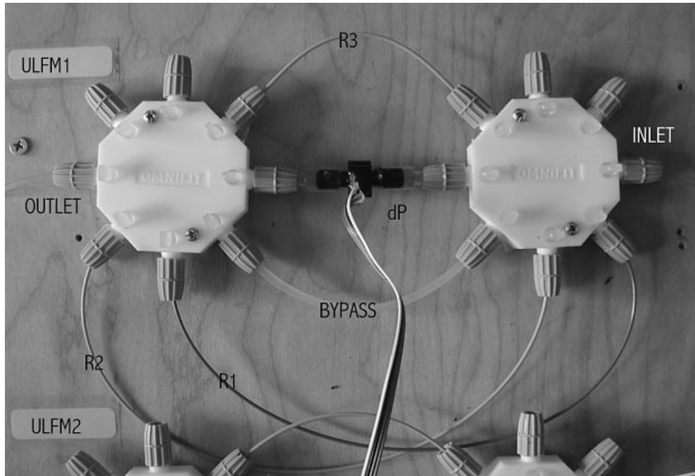
Fig. 2. Pictured is one of two Ultra-Low Flowmeters (ULFM) mounted on plywood. Water flows from the INLET to the OUTLET through two Omnifit 8-way valves (catalogue number U-06473-12, Cole-Parmer, Vernon Hills, IL). Valves are adjusted so water flow is through one of three ranges determined by the ID and length of PEEK tubing (i.e. tubes range from R1 through R3: R1=0.13 mm ID by 28 cm long, R2=0.18 mm ID by 28 cm, R3=0.18 mm ID by 9.5 cm) and the pressure drop across the range tube is measured with a differential pressure transducer ( dP =PX26-005DV, Omega Engineering, Stamford, CT). The BYPASS is 1.5 mm ID hard nylon tubing used for rapid filling of the system with water and for zero dP pressure checks. The four wires to dP provide power and send the signal to a datalogger connected to a computer. Although the pressure range of dP is 0–35 kPa, only the lower 0–5 kPa is used. During flow calibration dP was found to be reproducible to \pm 0.005 kPa, a long-term zero drift of about 0.05 kPa d^{-1} has been observed, but has little impact on measurements which typically required 10–20 min for seven measurements of flow at different suction pressures. The outlet tubing is 1 mm ID PEEK tubing connected to a compression fitting with custom cut rubber seals (catalogue number U-06473-07, Cole-Parmer). a PX26-001DV transducer with a dP range of 0–7 kPa was also used, but the zero drift and repeatability is about the same as the PX26-005DV and is more easily damaged by over-pressurization.
