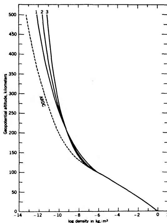
FIGURE 2.—Density-altitude relations for the model atmospheres.
