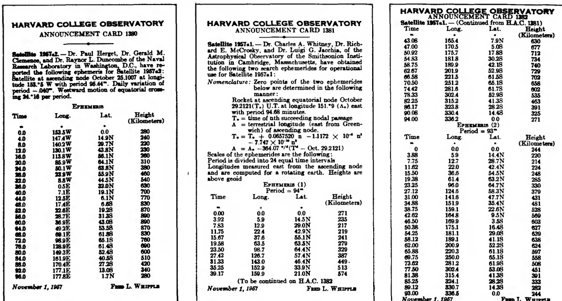
FIGURE 1.—Harvard Announcement Cards giving preliminary information on orbital characteristics for Satellites 1957 α1 and α2 (for No. 1381, note that from additional observations, Dr. C. A. Whitney obtained on Nov. 2, 1957, a refined value for the coefficient of the cubic term, i. e., 1.162 \times 10^{-9} instead of 7.747 \times 10^{-10} ).
