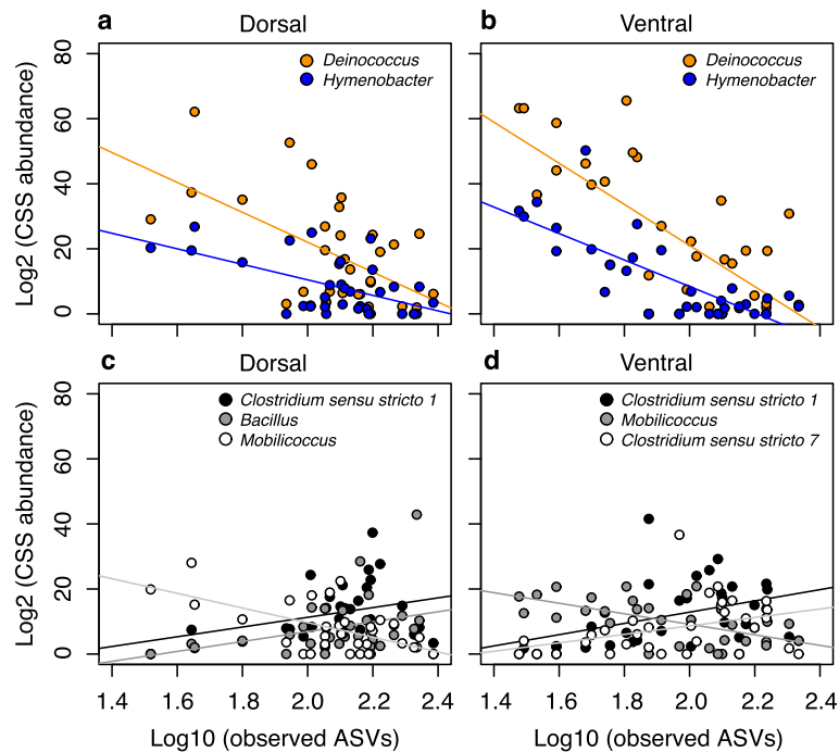
Fig. 5 Abundance of the commonest bacterial genera. Scatterplots of CSS \log_2 normalized counts of the commonest bacterial genera and the number of ASVs observed in plumage samples. a Deinococcus (adjusted R^2 = 0.30 , P = 0.0006 ) and Hymenobacter (adjusted R^2 = 0.30 , P = 0.0001 ) in dorsal plumage samples. b Comparable scatterplots for ventral plumage: Deinococcus (adjusted R^2 = 0.52 , P = 0.000001 ) and Hymenobacter (adjusted R^2 = 0.59 , P = 0.000001 ). c Scatterplots of the second ( Clostridium sensu stricto 1; adjusted R^2 = 0.10 , P = 0.043 ), fourth ( Bacillus ; adjusted R^2 = 0.10 , P = 0.041 ), and fifth most abundant genus ( Mobilicoccus ; adjusted R^2 = 0.35 , P = 0.0001 ) in dorsal plumage samples. d Comparable scatterplots for ventral plumage: Clostridium sensu stricto 1 (adjusted R^2 = 0.16 , P = 0.012 ), Mobilicoccus (adjusted R^2 = 0.33 , P = 0.0003 ), and Clostridium sensu stricto 7 (adjusted R^2 = 0.13 , P = 0.024 ). The x-axis represents the number of ASVs ( \log_{10} ) observed in individual samples. R^2 and two-tailed P -values were derived from simple linear regression
