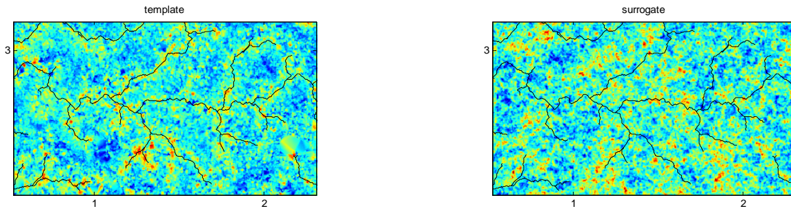
Figure S2. A map of MCH and the drainage network in a 180-ha subset of the study area (left), together with an example of an IAAFT surrogate for the same area. Note that the surrogate preserves the spatial structure in MCH observed in the original, but the correlation with the drainage network (black lines) is lost.
