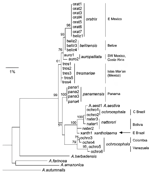
FIG. 3. Phylogram of the Amazona ochrocephala complex obtained in a Bayesian analysis of the COI data set (622 bp). The tree represents a 50% majority-rule consensus of 464 trees generated by MRBAYES during an MCMC search (see text), and numbers at nodes are posterior probabilities. The tree was rooted using A. amazonica , A. autumnalis , A. barbadensis , and A. farinosa as outgroups. Current subspecies groupings (e.g. Forshaw 1989, Juniper and Parr 1998) and geographic origin of samples are indicated to the right of sample names.
