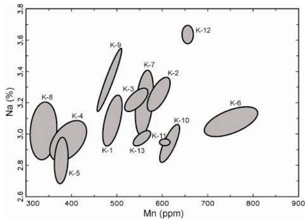
Fig. 1. Plot of Na versus Mn concentrations for obsidian from the Kamchatka region measured by NAA. Ellipses represent the 95 percent confidence interval for group membership.
