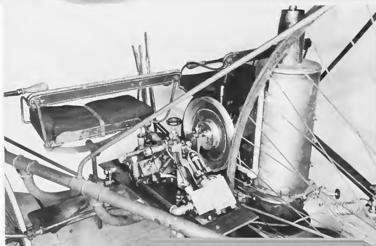
This steam tricycle, built by George A. Long about 1880, has been restored and is operable, but some of its parts are modern replacements. Below, left side, showing details of the 2-cylinder, V-type steam engine.
