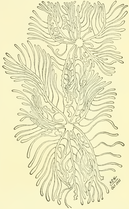
FIG. 162.—GALLERIES OF A SCOLYTID BEETLE. PITयोगENES CARINICEPS .
