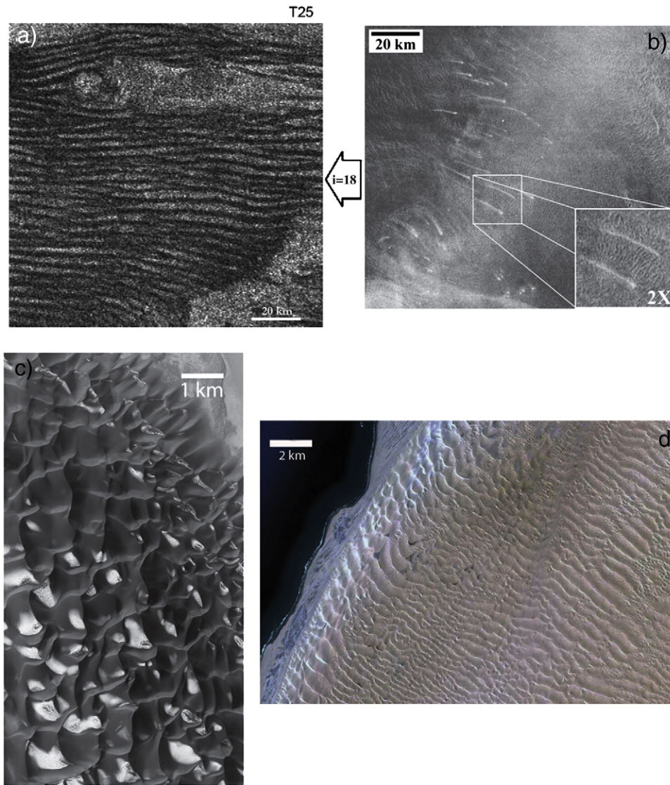
Fig. 1. Examples of planetary dune fields. a) Dunes on Titan are seen in this Cassini Radar image as dark lines overlying a bright substrate. The dunes are seen to divert around topographic obstacles, evident as bright/dark pairs in the Radar image and sand-free inter-dunes are also evident. The image was obtained February 22, 2007 at 300 m resolution near 10°N and 30°W. b) Fortuna-Meshkanet dune field on Venus. Portion of Magellan SAR F-Map 66N084, with effective resolution of ~100 m/pixel. 2× enlargement shows dune ridges transverse to the orientation of wind streaks, consistent with the formation as aeolian bedforms. c) Transverse dunes in a southern hemisphere crater on Mars (47.2°S; 34°E). High albedo areas are remnant patches of seasonal CO 2 frost. HiRISE image PSP_010854_1325, 50.9 cm/px. d) Transverse dunes in the Cunene Sand Sea, Namibia (17°23′25.54″S; 11°50′58.55″E). Mission data for the various bodies are available from: Titan: http://saturn.jpl.nasa.gov/index.cfm . Mars and Venus: http://pdsmaps.wr.usgs.gov/maps.html . Mars: searchable map database: http://themis.asu.edu/maps . Image d courtesy of Google Earth.
