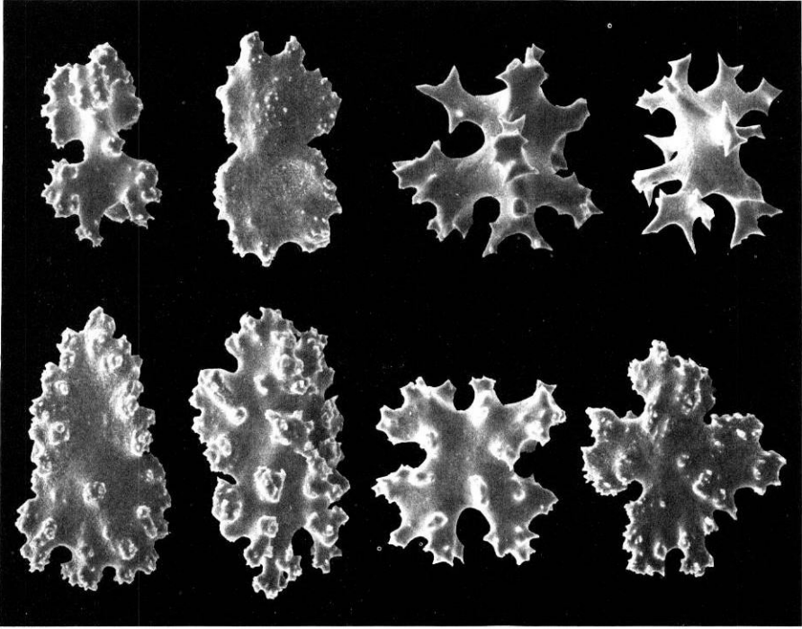
Fig. 3. Sarcodictyon catenatum . Sclerites, \times 325 .
