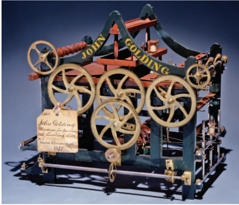
Patent No. 352. John Golding. Machine for Doubling and Twisting Thread. August 16, 1837. (SI neg. 86-5800)
