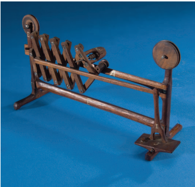
Patent No. 154,969. Walter B. Walker. Spinning Wheel. September 15, 1874. Arms contracted. (SI neg. 2009-11199)
