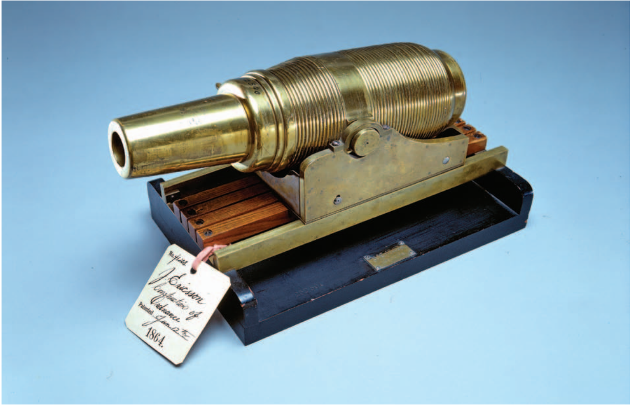
Patent No. 41,208. John Ericsson. Ordnance Construction. January 12, 1864. (SI neg. 85-18094)
