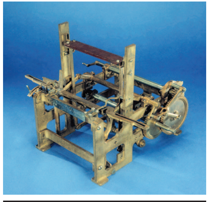
Patent No. 177,920. Erastus B. Bigelow. Carpet Loom. May 30, 1876. (SI neg. 89-6651)
