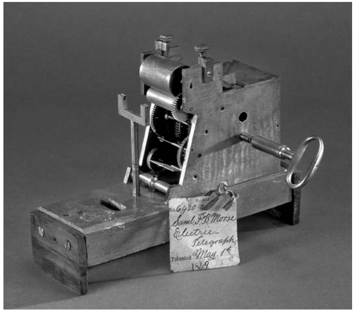
Patent No. 6,420. Samuel F. B. Morse. Electric Telegraph. May 1, 1849. (SI neg. 89-6904)
