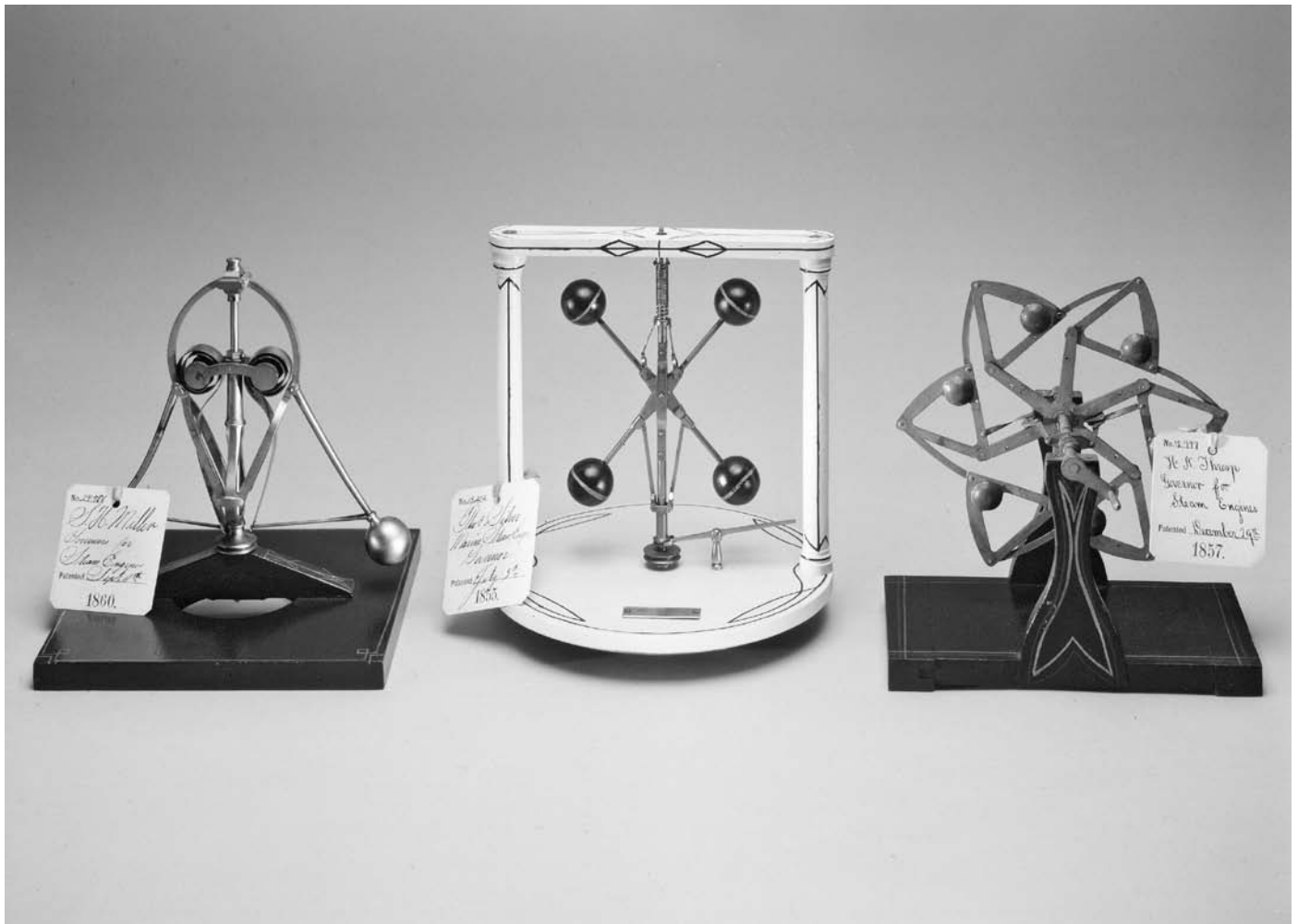
Left: Patent No. 29,986. S. H. Miller. Steam Engine Governor. September 11, 1860. Center: Patent No. 13,202. Thomas Silver. Steam Engine Governor. July 3, 1855. Right: Patent No. 18,997. H. N. Throop. Steam Engine Governor. December 29, 1857. (SI neg. 83-13267).
