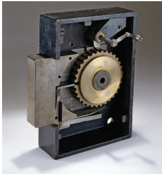
Patent No. 32,330. Linus Yale, Jr. Lock. May 14, 1861. (SI neg. 86-6336)
