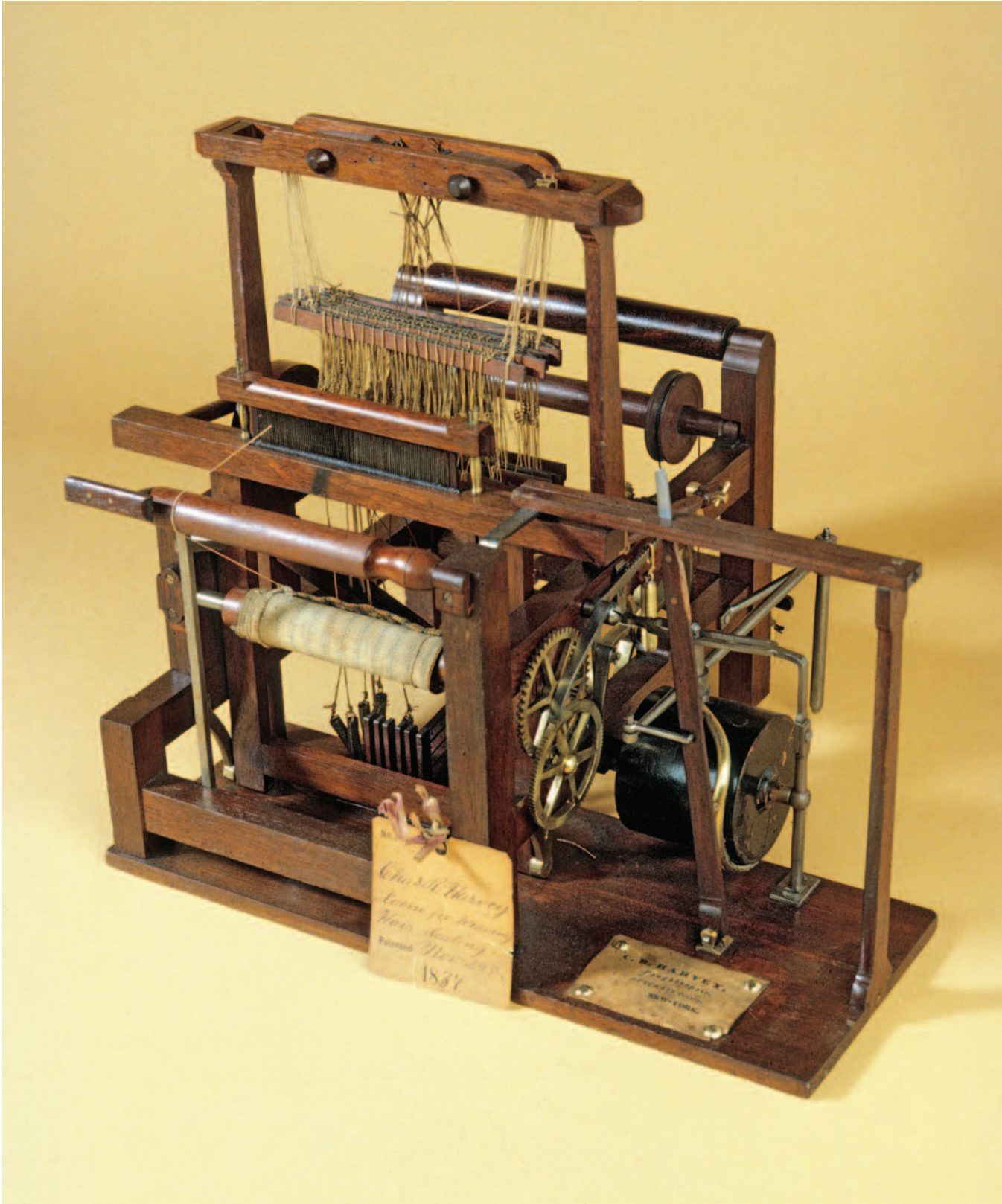
Patent No. 490. Charles R. Harvey. Hair Cloth Loom. November 25, 1837. (SI neg. 80-16793)
