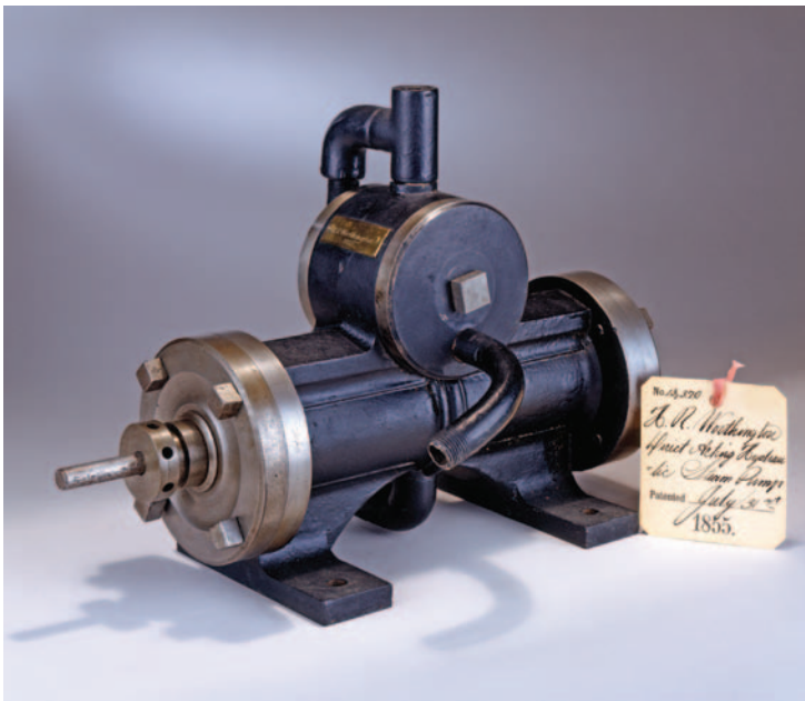
Patent No. 13,370. Henry R. Worthington. Direct Acting Steam Pump. July 31, 1855. (SI neg. 86-6334)
