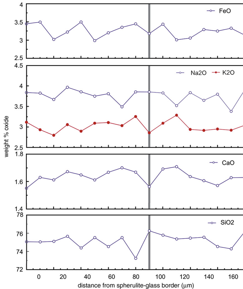
Fig. 2. Major element compositions of glass leading up to a spherulite margin (at position = 0 \mu\text{m} ). All analyses were collected with an electron probe microanalyzer. The vertical grey bars demarcate the approximate ( \pm 10 \mu\text{m} ) position of the colorless–brown glass boundary.
