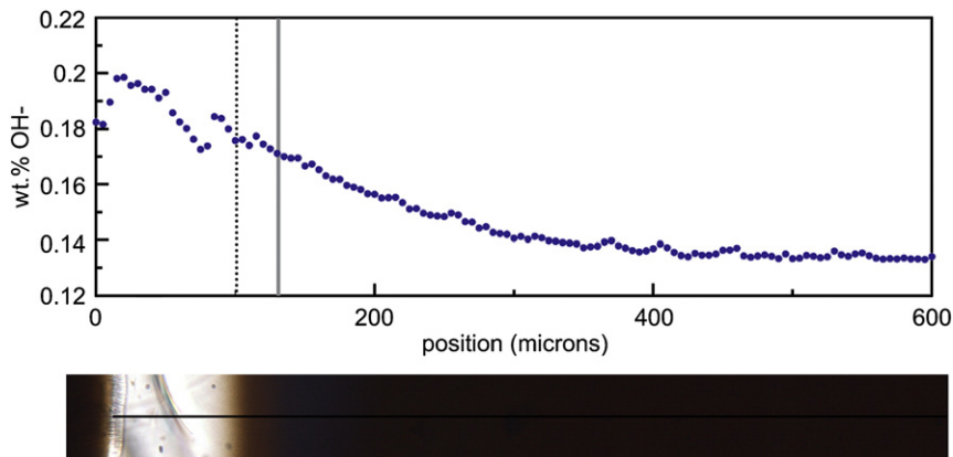
Fig. 6. An \text{OH}^- concentration profile measured along a traverse extending from a spherulite in the heated obsidian sample. The position of traverse is shown on the subjacent photomicrograph. The vertical dashed and solid grey lines on the profile bound the light brown glass zone that may have formed as a result of degassing of hydrogen into the crack shown in the photomicrograph. Note the coincidence between the depression in the \text{OH}^- concentration profile and the position of the crack at \sim 75 –80 \mu\text{m} .
