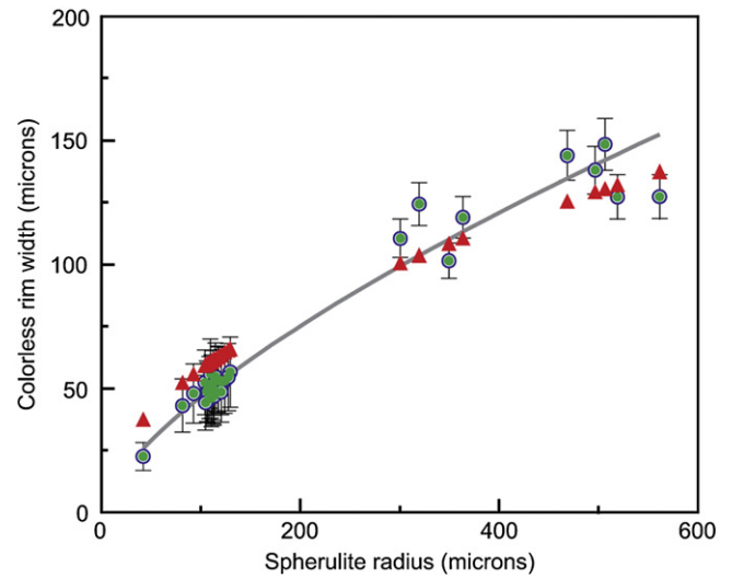
Fig. 4. Colorless glass rim width versus the apparent spherulite radius, measured on photomicrographs of the Krafla obsidian (solid dots). Error in rim width, shown as vertical bars, ranges from about 10 to 20%, and originates from the diffuse nature of the colorless–brown glass boundaries. Regression curve is a power law function of the form: y = 2x^{0.69} ; R^2 = 0.97 . Solid triangles are the predicted rim widths based on the experimentally constrained hydrogen–iron reaction rate constant of Gaillard et al. (2003b), and the assumption that the rims developed during the interval of time that the spherulites grew, which in turn, is taken from the growth rate data of Castro et al. (2008).
