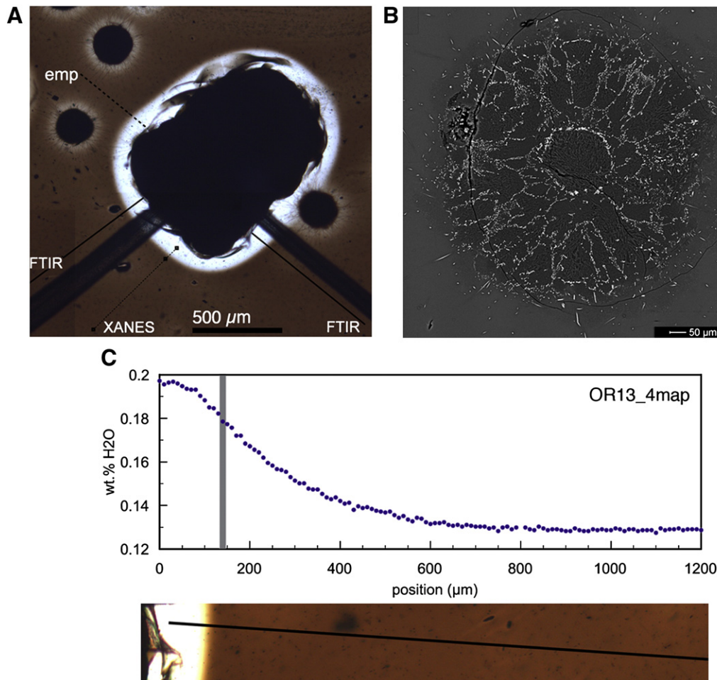
Fig. 1. A) Photomicrograph of spherulites (round and elliptical, black) in obsidian (brown). Various analytical points and traverses are shown (emp = electron probe microanalyzer; FTIR = Fourier Transform Infrared Spectroscopy; XANES = X-ray absorption near-edge spectroscopy). Black diamonds indicate approximate locations of \mu -XANES measurements. Broader dark swaths are tracks left by a laser ablation ICPMS (these data are not discussed here). B) A backscattered electron image showing typical internal spherulite texture. Bright phases are clinopyroxene and magnetite. C) An \text{OH}^- concentration profile determined by FTIR collected along the lower right traverse in frame A. The vertical grey line is the approximate location of the colorless–brown glass boundary. (For interpretation of the references to colour in this figure legend, the reader is referred to the web version of this article.)
