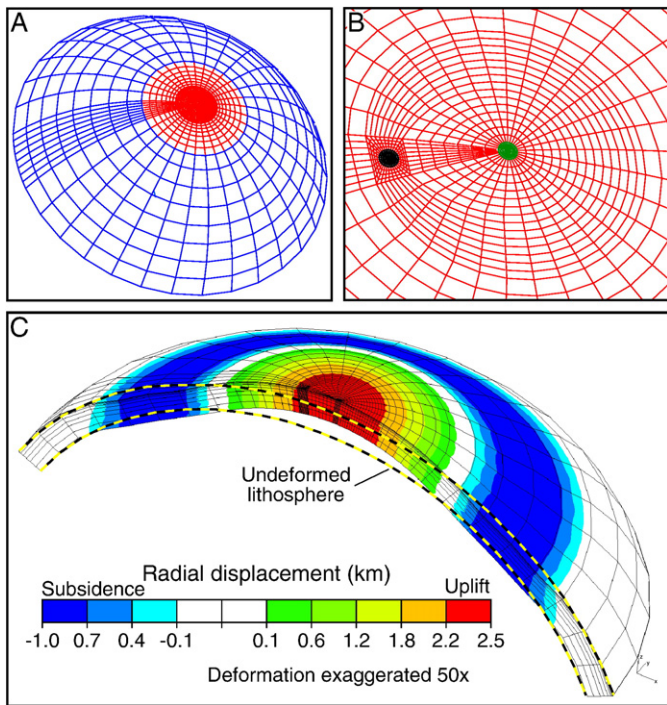
Fig. 2. (A) 3-D spherical finite element model covering a cap extending radially to 80^\circ of arc and to a depth of 400 km; the 1500-km-diameter Caloris basin is shown in red. Element size decreases toward the basin center to provide greater resolution in this region. (B) Close-up of basin center showing the \sim 40 -km-diameter Apollodorus crater (green) at the center of Caloris basin and a similar-sized crater (black) offset 200 km from the basin center. (C) Calculated deformation of Mercury's lithosphere due to loading associated with the external smooth plains assumed to completely surround the Caloris basin between radial distances of 850 and 1850 km from the basin center. Subsidence of the smooth plains is shown in cool colors, while the resulting uplift of Caloris basin is shown with warm colors.
