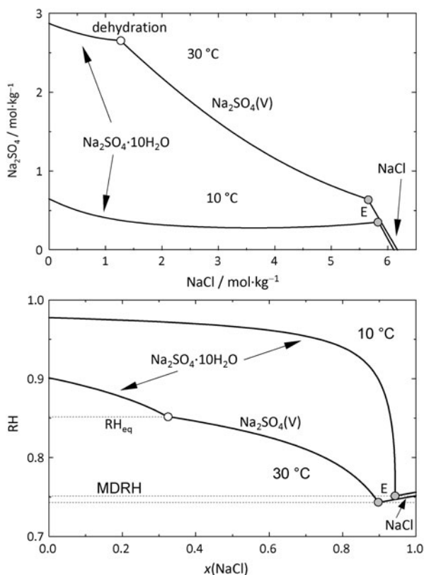
Fig. 4.27 Solubilities (a) and saturation humidities (b) in the NaCl–Na 2 SO 4 –H 2 O system at 10°C and 30°C
