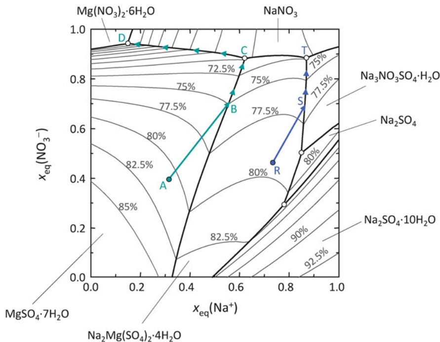
Fig. 4.29 Solubilities and saturation humidities in the system \text{Na}^+ - \text{Mg}^{2+} - \text{NO}_3^- - \text{SO}_4^{2-} - \text{H}_2\text{O} at 25^\circ\text{C} . Adapted from Steiger et al. (1998)
