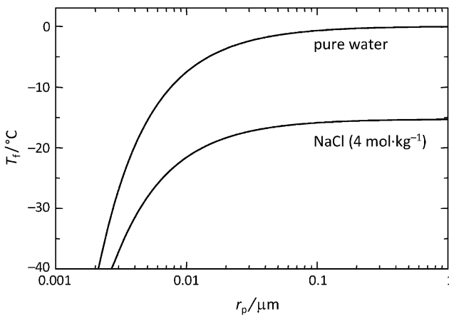
Fig. 4.11 Freezing temperatures T_f in water and aqueous NaCl as a function of pore size in a saturated porous material. Adapted from Steiger (2006b)
