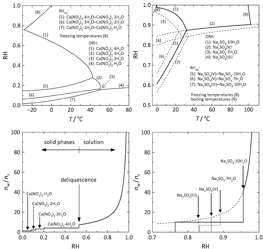
Fig. 4.25 RH/T phase diagram (top) and water uptake curves (bottom) of \text{Ca(NO}_3)_2\text{--H}_2\text{O} (left) and \text{Na}_2\text{SO}_4\text{--H}_2\text{O} (right); dashed curves represent metastable equilibria
