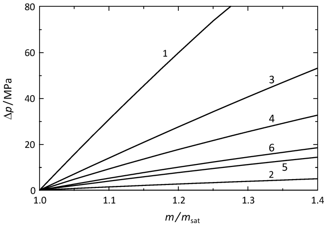
Fig. 4.10 Crystallization pressures at 25°C in supersaturated solutions of (1) NaCl (halite), (2) Na 2 SO 4 ·10H 2 O (mirabilite), (3) Na 2 SO 4 (thenardite), (4) NaNO 3 (nitratine), (5) MgSO 4 ·7H 2 O (epsomite) and (6) MgSO 4 ·6H 2 O (hexahydrate). Adapted from Steiger (2005a); supersaturation is expressed as the ratio of the molality m of the supersaturated solution and the saturation molality m_{\text{sat}} of the respective salt
