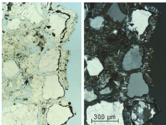
Fig. 4.14 Thin section of gypsum crust on a quartz bound sandstone at Leineschloss (Hanover) with // Nicols ( left ) and X Nicols ( right ). Note the loss of cohesion of the surface quartz grains due to secondary gypsum growth. The gypsum crystals growing on the original thin black surface layer resulted from the subsequent development of a leak above this area. Reproduced with permission from Neumann et al. (1993)
