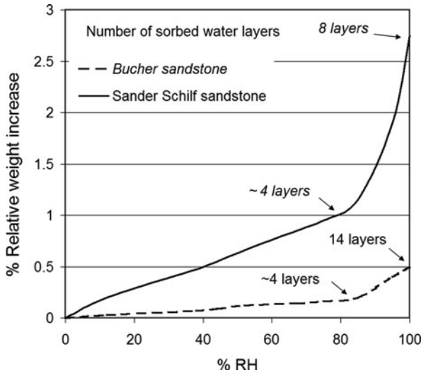
Fig. 4.6 Water sorption curves for the coarse-pore Bucher and mixed-pore Sander Schilf sandstone that also contains more phyllosilicates. Adapted and simplified from Sneath 1984. The number of sorbed water layers was calculated based on the amount of sorbed moisture that in turn reflect the specific surface area of the stones (2.63 and 14.8 m 2 /g, respectively). Note that at the inflection point of the curve (approx. 80% RH) both stones had absorbed the same number of water layers
