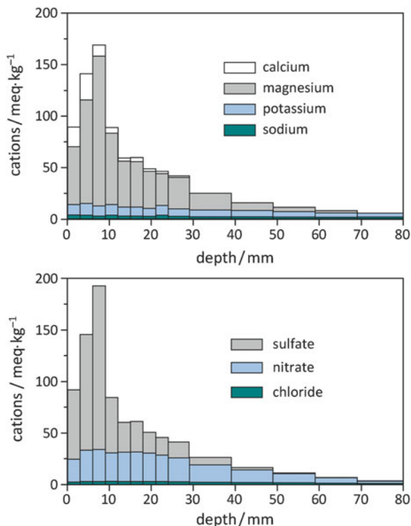
Fig. 4.22 Salt profile in sandstone from Schloss Weissenstein, Pommersfelden. Adapted from Steiger (2003)
