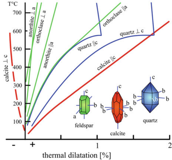
Fig. 4.2 Linear expansion changes for some minerals as a function of temperature. Adapted from Winkler 1994
