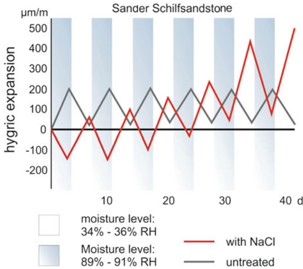
Fig. 4.13 Hygric expansion for a Sander Schilf sandstone sample and for one pre-treated with a NaCl solution. Adapted from Snethlage and Wendler (1997)
