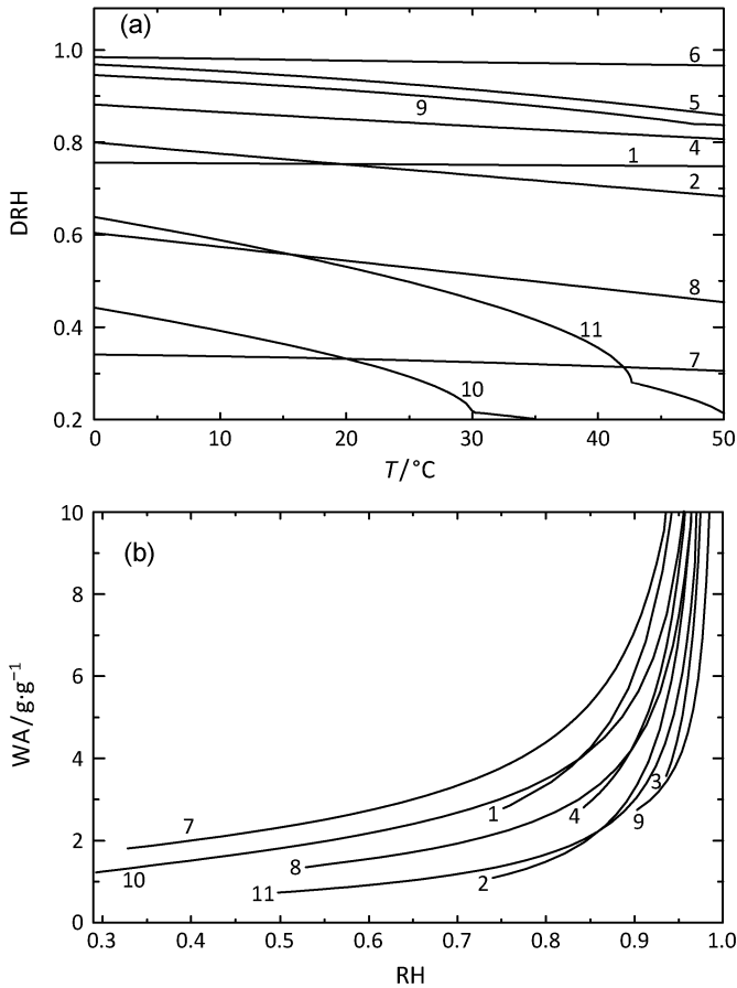
Fig. 4.24 Deliquescence humidities (a) and hygroscopic moisture uptake (b) of several salts commonly found in building materials: (1) NaCl, (2) NaNO 3 , (3) Na 2 SO 4 , (4) KCl, (5) KNO 3 , (6) K 2 SO 4 , (7) MgCl 2 ·6H 2 O, (8) Mg(NO 3 ) 2 ·6H 2 O, (9) MgSO 4 ·7H 2 O, (10) CaCl 2 ·6H 2 O, (11) Ca(NO 3 ) 2 ·4H 2 O
