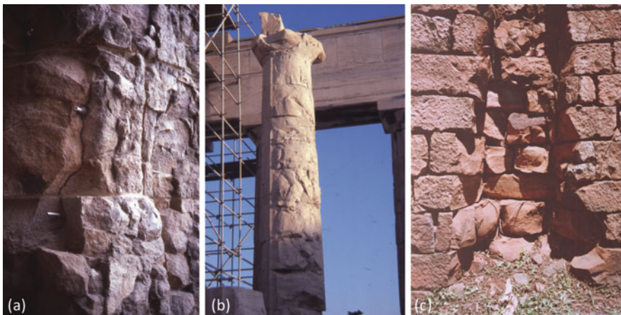
Fig. 4.1 Detail of the conchoidal fractures resulting from historic fires: (a) granite pillars in the former Custom Building, now a market, in Salvador, Bahia, Brazil; (b) marble columns of the Parthenon, Athens, Greece; (c) niche for a wooden column in the church wall constructed with argillaceous sandstone in the Jesuit Guaraní Mission of Santa Ana, Misiones, Argentina
