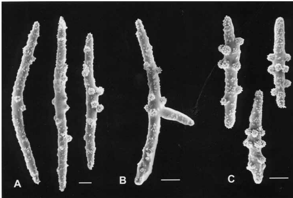
Fig. 3. Alectona millari Carter, holotype BMNH 82.4.27.4. SEM view of spicules. A, small acanthocheas. B, acanthotriactine. C, spiny microstrongyle, transition to amphiasters (scale 10 \mu\text{m} ).
