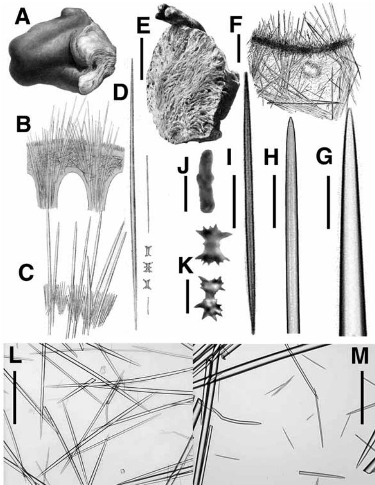
Fig. 9. Scolopes , spiculation and habitus. A–D, S. moseleyi Sollas. A, habitus. B, choanosomal skeletal structure. C, ectosomal palisade and hispidation. D, spiculation. E–M, S. lignea (Hallmann). E, habitus (scale 40 mm). F, choanosomal skeletal structure (scale 300 \mu\text{m} ). G, tip of large choanosomal oxea (scale 60 \mu\text{m} ). H, tip of medium sized subectosomal oxea (scale 30 \mu\text{m} ). I, small oxea of ectosomal palisade (scale 20 \mu\text{m} ). J, granular microtrich (scale 10 \mu\text{m} ). K, amphiasters (scale 5 \mu\text{m} ). L, large choanosomal oxeas (scale 500 \mu\text{m} ). M, small and medium sized ectosomal oxeas (scale 100 \mu\text{m} ). (A–D, after Sollas, 1888, pl. XLIII. E–F, after Hallmann, 1912, fig. 27, pl. xxii fig. 2.)
