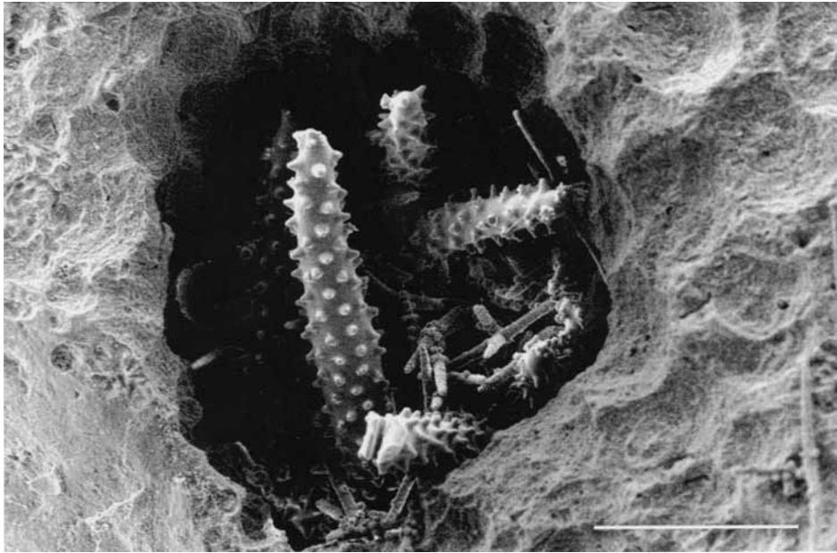
Fig. 2. Alectona millari Carter, holotype BMNH 82.4.27.4. SEM view of substrate excavation with large acanthochea protruding (scale 100 \mu\text{m} ).
