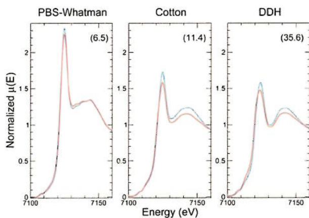
Fig. 8 Normalised XANES spectra of unfaded (blue) and faded (red) Prussian blue artefacts on paper (PBS-Whatman), textile (cotton) and gelatin (DDH) samples. \Delta E values are indicated in parentheses at the top of each XANES spectrum.
