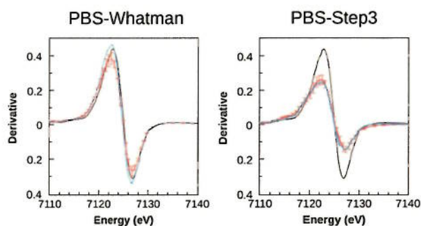
Fig. 3 Derivatives of the XANES absorption spectra illustrating the broadening of the absorption edge for PBS– Whatman and PBS– Step3 samples. Powder (black) and PBS–paper samples before (blue) and after fading (red). Errors bars correspond to standard deviations on 4 and 5 measurements for PBS– Whatman and PBS– Step3 respectively.
