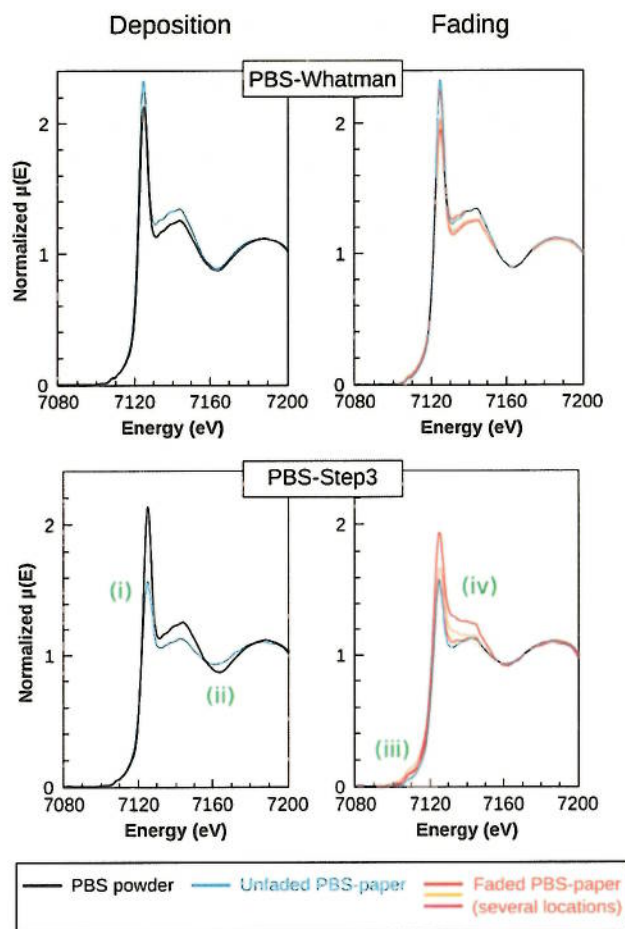
Fig. 2 XANES spectra of PBS powder (black) and PBS-paper samples before (blue) and after fading (red-orange). Due to heterogeneity observed in the faded PBS-paper samples, measurements were performed at three to five different locations of each sample (red-orange curves). For PBS-Step3 samples, structural variations are observed both before and after light exposure and occur in four regions of the spectra denoted (i)–(iv).
