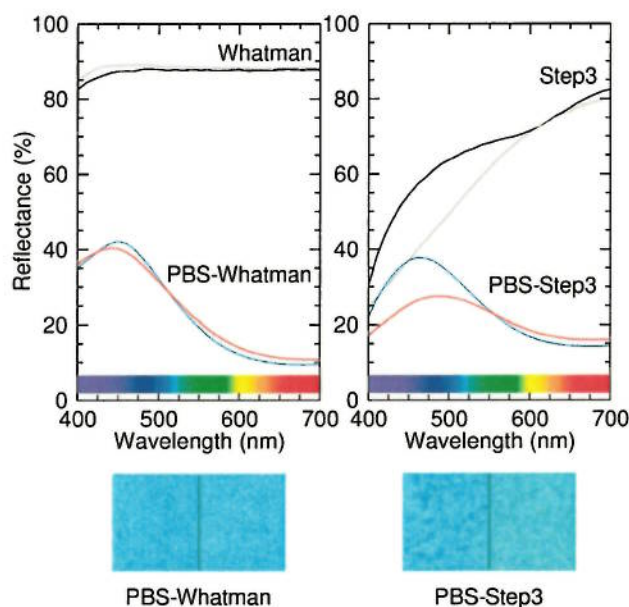
Fig. 4 Reflectance curves of PBS–paper samples before (blue) and after fading (red). For reference, reflectances curves of papers alone before (black) and after fading (gray) are indicated. Bottom: optical photographs of the unfaded and faded samples (respectively left and right parts of the photographs).
