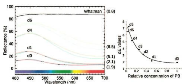
Fig. 6 Left: reflectance curves of PBS-Whatman paper systems at different PB concentrations, before (blue shades) and after fading (red shades). Values in brackets refer to \Delta E values. For reference, the reflectance curve of Whatman alone before (black) and after fading (gray) is indicated. Right: relative PB concentration vs. \Delta E , showing the entire relative concentration series [d0–d6]. Data could be fitted with an exponential law of the kind a + \exp^{-x/b} (plain line).
