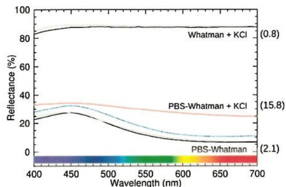
Fig. 5 Reflectance curves before (blue) and after fading (red) of PBS- Whatman systems enriched in KCl. Values in brackets refer to \Delta E values. Control reflectance curves before and after fading of Whatman paper enriched in KCl and PBS- Whatman without KCl (sample d1) are indicated in black and gray, respectively.
