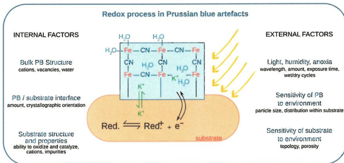
Fig. 9 Summary of internal and external factors playing a role in the redox processes in Prussian blue–substrate systems. In this paper, we have particularly emphasized on the impact of “Bulk PB structure” and “Substrate structure and properties” on the fading behavior of model PB–paper systems. The impact of “Light, humidity, anoxia” was partly investigated on similar PB–paper systems by Gervais et al. 18
