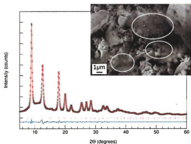
Fig. 1 Diffraction pattern of PBS at 293.0 K, \lambda = 0.7931 Å (cross), its LeBail fit (line) and residues (vertical bars mark the Bragg reflection). Inset: SE-SEM image of PBS powder (working distance: 2 mm; accelerating voltage: 0.5 kV, p = 5 \times 10^{-7} mbar). Circles indicate regions where distinct nanoparticles may be observed.
