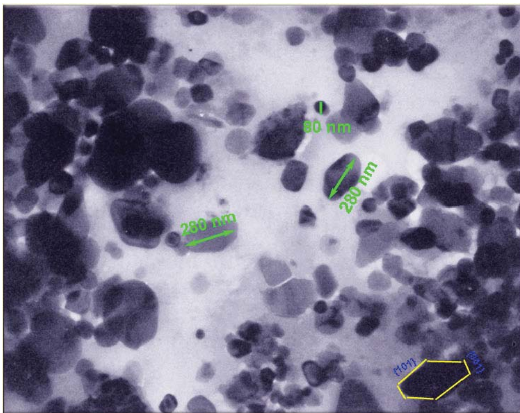
Figure 1. Transmission electron micrograph of anatase particles from the ink of the Vinland Map (reproduced from Figure 2 of Towe 1990). Labeled particle sizes are estimated using the reported image magnification and the image dimension for the figure from Towe, 1990. Anatase particles present the equilibrium morphology of truncated tetragonal bipryamids as indicated by green arrows. Seemingly spherical smaller particles are likely of the same shape, but this is hard to confirm due to limited image resolution. Particles with lower image contrast (grayer) may be other minerals whose cations have lower atomic numbers than titanium (e.g. calcite, or quartz). Reprinted with permission from Towe, K.M., Acc. Chem. Res. , 1990 , 23, 84-87. Copyright 1990 American Chemical Society.
