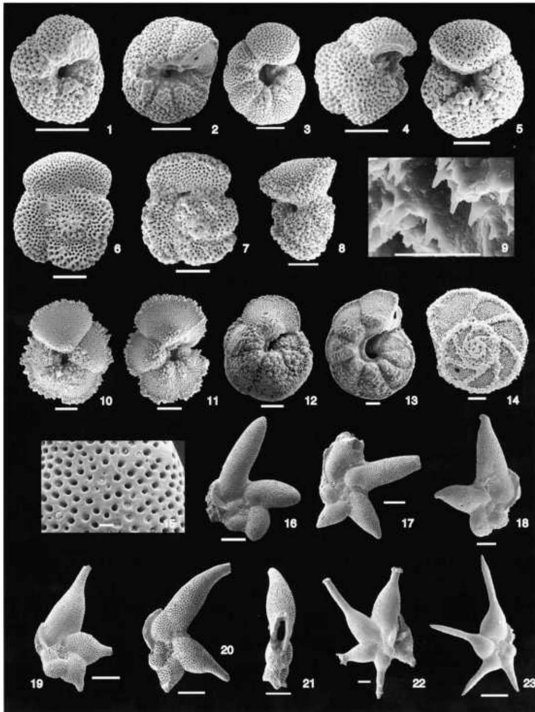
Plate 2. Selected planktonic foraminifera from TDP Site 2. Scale bars = 100 µm, except where given. (1) Igorina lodoensis (Sample TDP2/28/2, 16–24 cm); (2) Igorina broedermanni (Sample TDP2/13/CC); (3) Igorina anapetes (Sample TDP2/17/2, 35–43 cm); (4) Acarinina cf. subsphaerica (Sample TDP2/9/CC); (5) Acarinina matthewsae (Sample TDP2/9/CC); (6) Acarinina matthewsae (Sample TDP2/9/CC); (7) Acarinina praetopilensis (Sample TDP2/19/1, 10–20 cm); (8) Acarinina praetopilensis (Sample TDP2/9/CC); (9) detail of ultra-fine sub-micron mural ornamentation in apertural system (scale bar = 1 µm); (10) Morozovella coronata (Sample TDP2/1/2, 50–57 cm); (11) Morozovella coronata (Sample TDP2/2/1, 16–26 cm); (12) Morozovella aragonensis (Sample TDP2/17/2, 35–43 cm); (13) Morozovella crater (Sample TDP2/14/2, 1–31 cm); (14) Morozovella crater (Sample TDP2/3/CC); (15) Wall texture of transitional Hantkenina sp. (Sample TDP2/19/1, 90–100 cm); (16) Clavigerinella caucasica (Sample TDP2/23/1, 0–10 cm); (17) Clavigerinella caucasica (Sample TDP2/19/CC); (18) transitional Hantkenina sp. (Sample TDP2/22/1, 53–62 cm); (19) transitional Hantkenina sp. (Sample TDP2/18/1, 41–52 cm); (20) transitional Hantkenina sp. (Sample TDP2/18/2, 50–60 cm); (21) same specimen as 20, apertural view; (22) Hantkenina mexicana (Sample TDP2/4/2, 65–73 cm); (23) Hantkenina liebusi (Sample TDP2/5/1, 80–88 cm).
