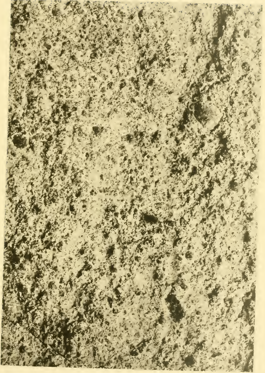
THE ALLEGAN METEORITE.
