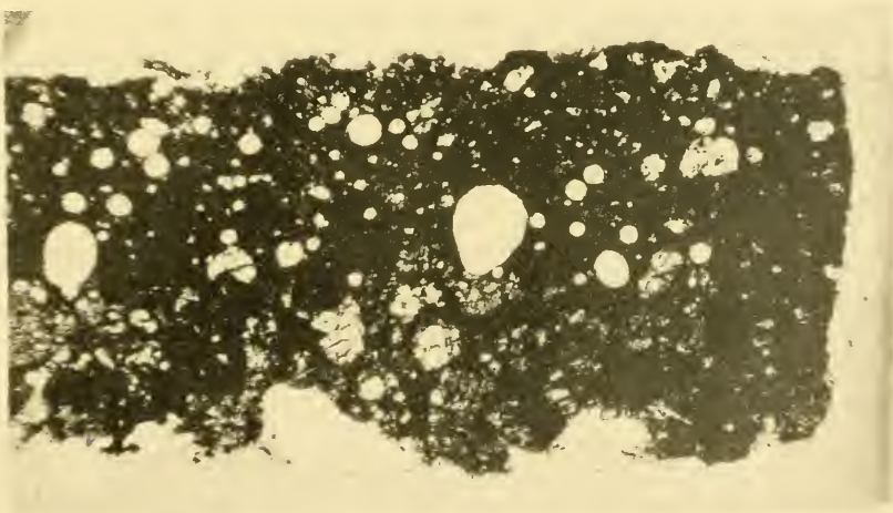
THE ALLEGAN METEORITE.
