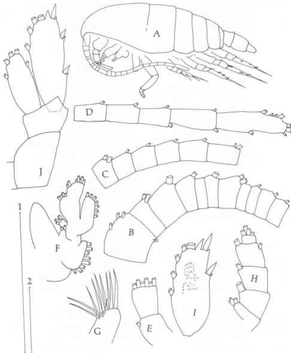
Fig. 7. Scopelatum vorax , CIII: A, animal, lateral; B, free segments 1-11 of A1; C, free segments 12-17 of A1; D, free segments 18-22 of A1; E, Mn, tip of Ri; F, Mx1; G, Mx1, armament of li1; H, end of basis and Ri of Mxp; I, Re1 of P3; J, P4. Line 1 = 1.0 mm for A; line 2 = 0.1 mm for B-J; letters on proximal-most segments of B-D.
