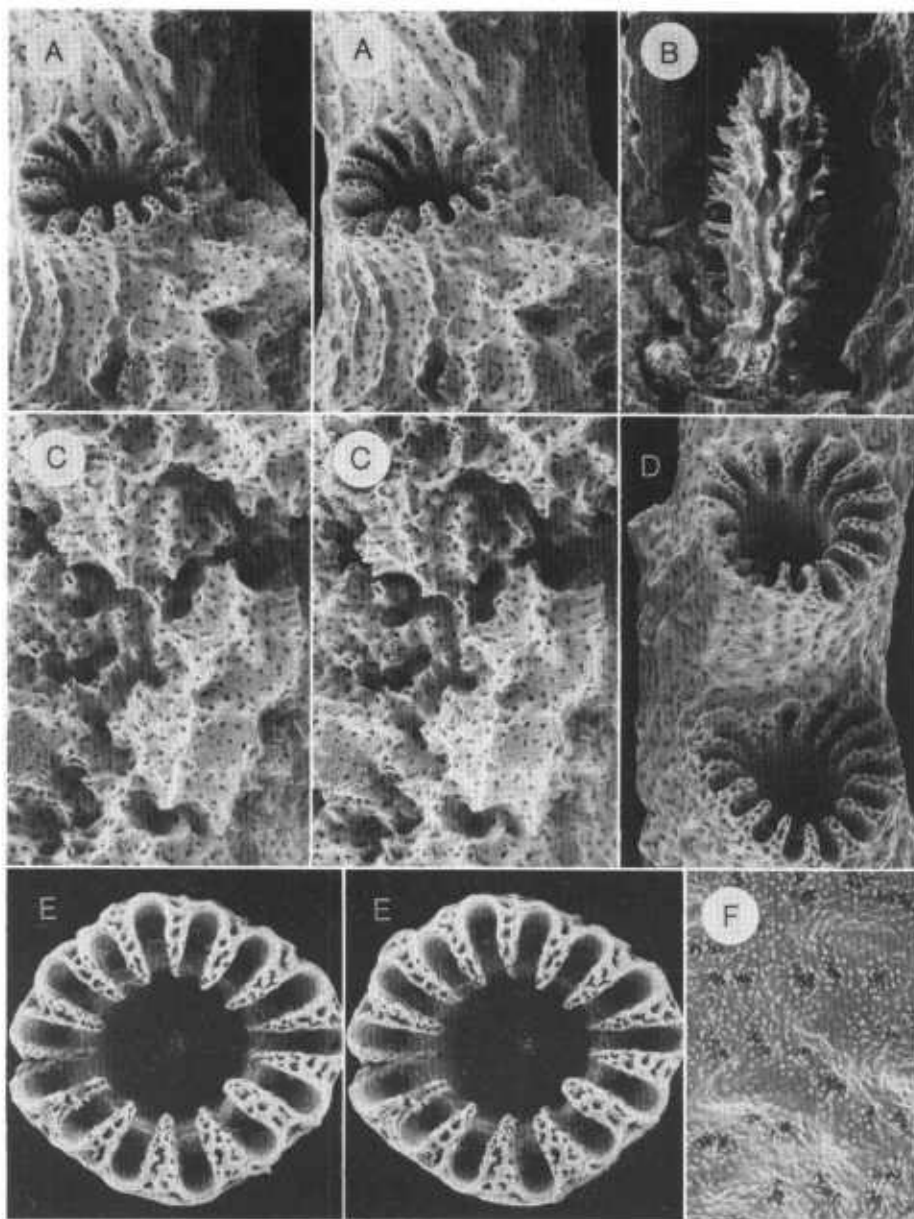
Figure 3 Stylander tenisonwoodsii sp. nov. Paratypes from WAM 934-86: A. Cyclosystem, carinate coenosteum and female ampullae, x 31.1, stereo pair. B. Gastrostyle and ring palisade, x 123. C. Cluster of female ampullae, x 32, stereo pair. D. Two cyclosystems, x 34.5. E. Cyclosystem including view of several lateral dactylostyles in upper dactylotomes, x 57, stereo pair. F. Coenosteal texture, x 111.
