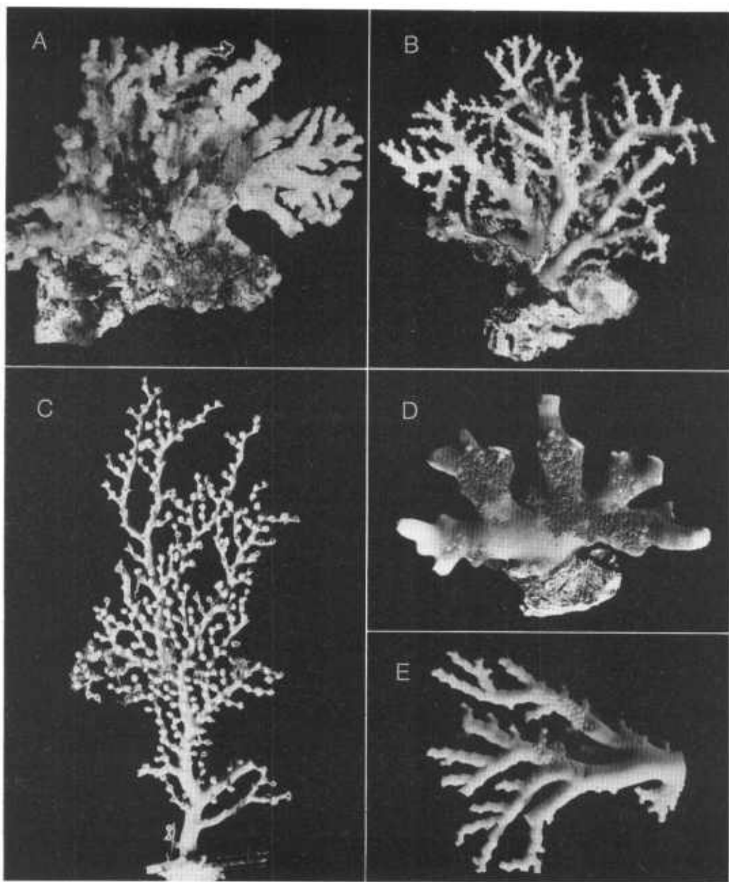
Figure 1 A. Styaster marshae sp. nov., holotype, WAM 535-87, x 0.73. B. Styaster tenison-woodsi sp. nov. holotype, WAM 536-87, x 1.2. C. Crypthelia pudica , WAM 19-85, male, x 1.1 D. Distichopora violacea , WAM 936-86, female, x 2.1. E. Styaster marshae sp. nov., paratype, female, USNM 79519, x 14.
