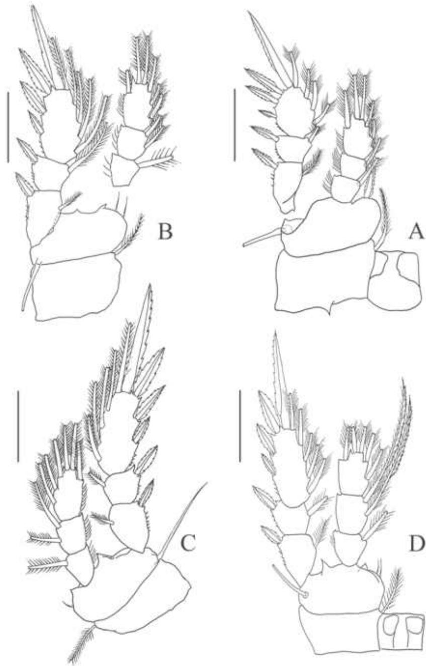
Fig. 10. Limnoithona tetraspina Zhang et Li, 1976. Male. A — leg 1, B — leg 2; C — leg 3; D — leg 4. Scale bars: A–D — 0.025 mm.
