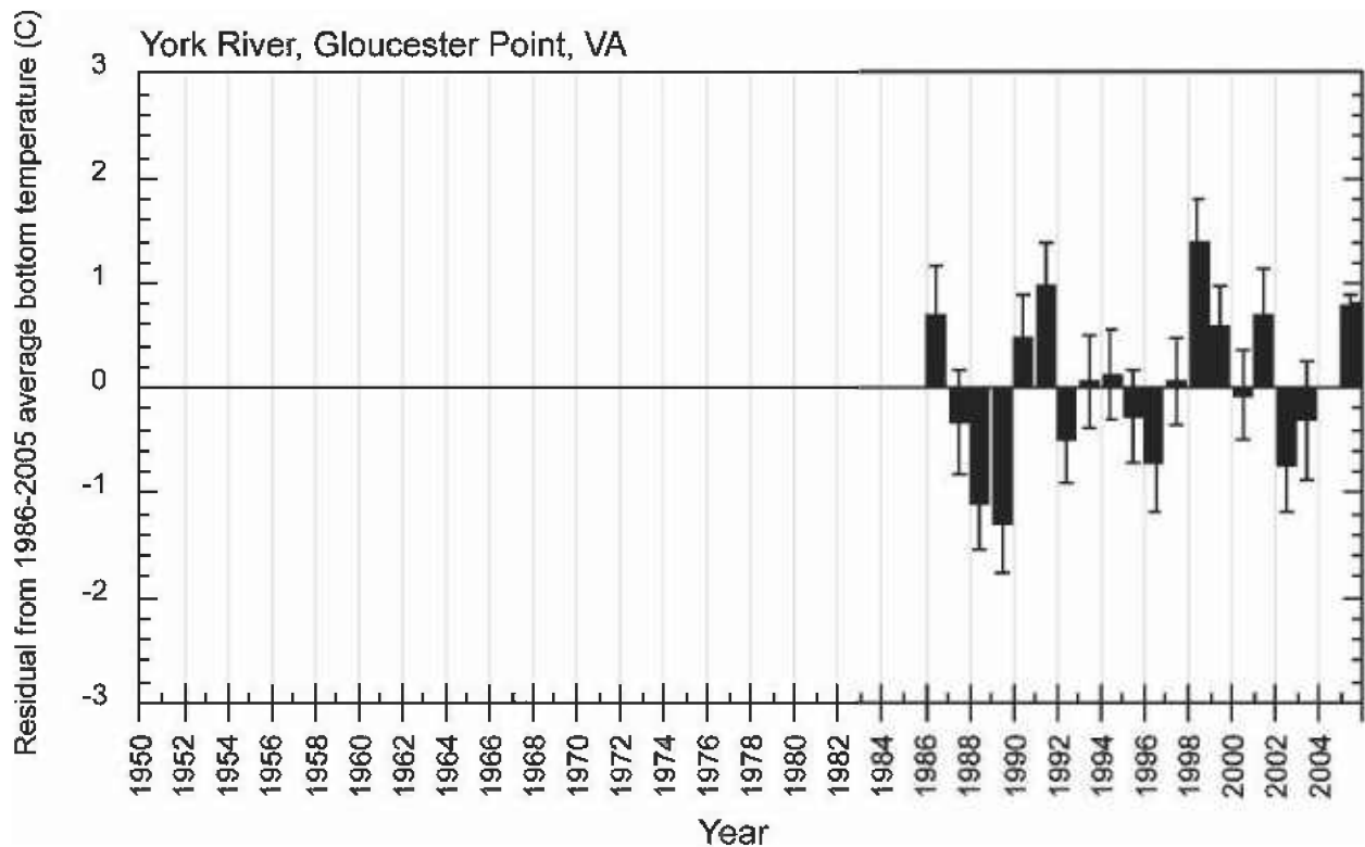
Figure 16. Annual average residual bottom temperature (BT) from the long term (1986–2005) average bottom temperatures (16.23 °C, standard error of the mean 0.56 °C) recorded at Gloucester Point, Virginia. The error bars represent the standard error of the mean in degrees Celsius.
