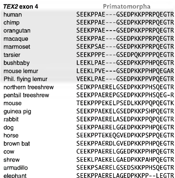
Fig. 1. An example of a coding sequence indel supporting the Primatomorpha hypothesis. A three-amino acid deletion in exon 4 of the TEX2 gene is present in all major primate lineages and both colugo genera (shaded gray) but is absent in all tree shrew lineages and eutherian outgroup representatives. See figs. S1 to S10 for full alignments and descriptions of additional supporting indels for Euarchonta and Primatomorpha.
