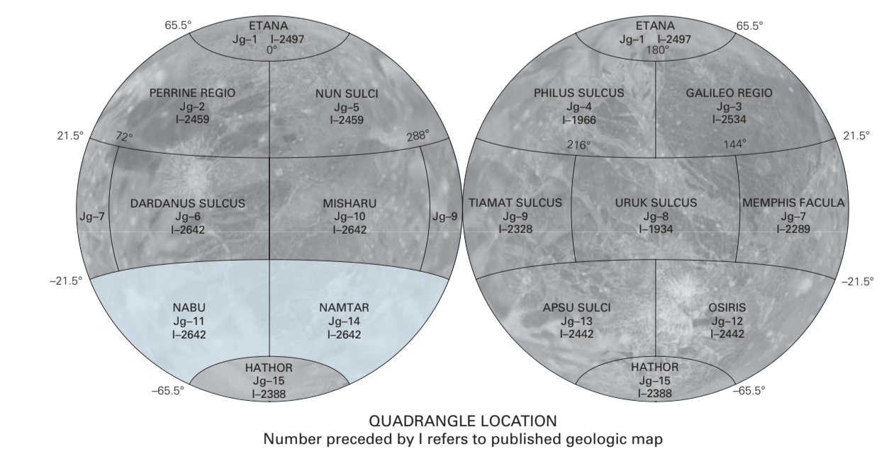
GEOLOGIC MAPS OF THE DARDANUS SULCUS (Jg-6), MISHARU (Jg-10), NABU (Jg-11), AND NAMTAR (Jg-14) QUADRANGLES OF GANYMEDE By Ted A. Maxwell and Ursula B. Marvin 2001
