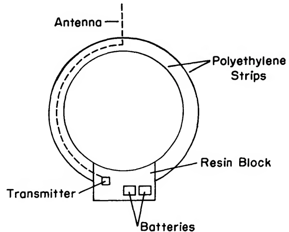
FIGURE 12.—Diagram of radio-collar.
