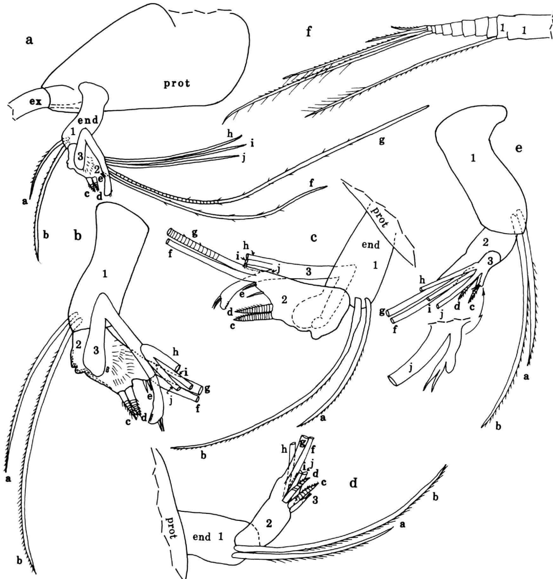
FIGURE 4.— Spelaeoecia cubensis , new species, paratype, USNM 194306, adult male: a, right 2nd antenna, mv; b,c, endopodite of right 2nd antenna, medial and lateral views, respectively; d,e, endopodite of left 2nd antenna, lateral and medial views, respectively; f, exopodite of left 2nd antenna (bristles of joints 2-7 not shown).
