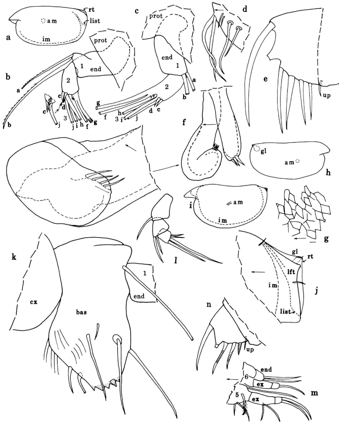
FIGURE 9.— Spelaeoecia cubensis , new species. USNM 194312, A-1 male, paratype: a, complete specimen from left side, length 1.55 mm; b, c, endopodites of left and right 2nd antennae, respectively, lv; d, part of basale of left mandible (drawn attached to body), lv; e, left furcal lamella, lv; f, distal part of copulatory organ. g, USNM 194313f, A-1 male, paratype, length 1.67 mm, indistinct surface reticulations near middle of left valve. h, USNM 194311, A-1 female, paratype, complete specimen from right side, length 1.62 mm. USNM 194310, A-4 instar (sex unknown), paratype: i, complete specimen from left side, length 0.67 mm; j, detail from i; k, part of right mandible, lv; l, part of left mandible, lv; m, distal parts of left 5th and 6th limbs (drawn attached to body), lv; n, left furcal lamella, lv.
