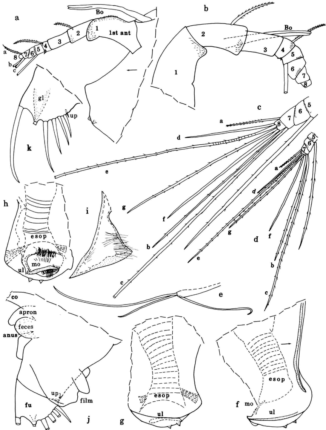
FIGURE 3.— Spelaeoecia cubensis , new species, paratype, USNM 194306, adult male: a , part of anterior of body from left side (bristles of joint 8 not shown); b , right 1st antenna, lv (bristles of joints 7 and 8 not shown); c, d , tip of left 1st antenna, lv; e , left 7th limb; f-h , anteroventral part of body from right side, anterior, and posterior, respectively; i , part of lower lip; j , part of posterior of body from left side; k , left furcal lamella, lv.
