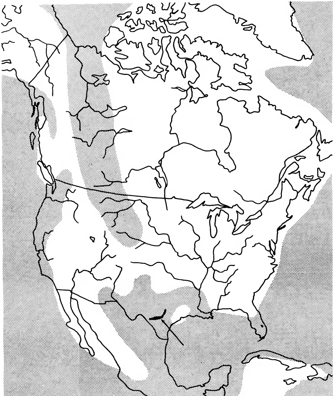
FIGURE 26.—Generalized paleogeographic map of North America showing marine transgression late in Early Cretaceous time (based on Dunbar, 1960:320). (Balcones Fault Zone superimposed and indicated by arrow; areas covered by marine water shaded.)
