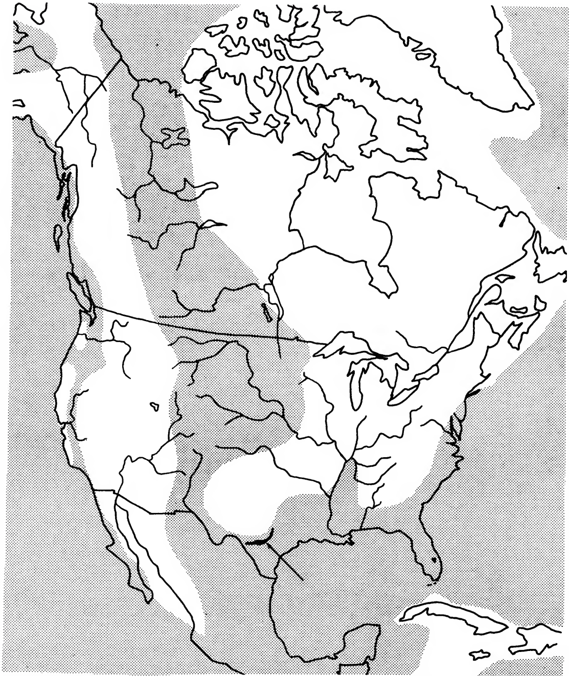
FIGURE 27.—Generalized paleogeographic map of North America showing maximum marine transgression in Middle to Late Cretaceous time (based on Dunbar, 1960:320 and Dott and Batten, 1976:357). (Balcones Fault Zones superimposed and indicated by arrow; areas covered by marine water shaded.)
