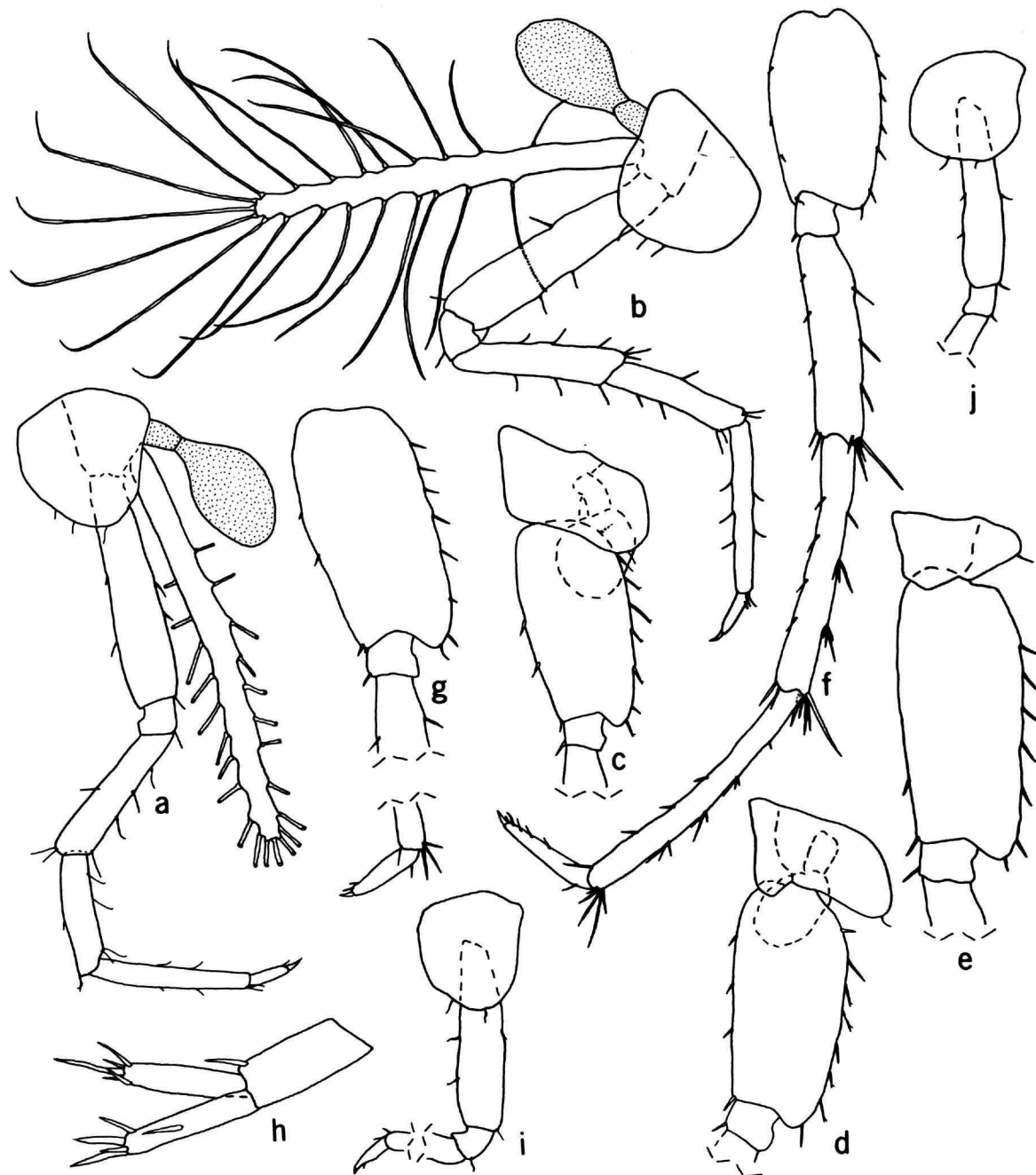
FIGURE 8.— Texiweckelia insolita , new species, paratypes, artesian well, Hays County, Texas, female (4.5 mm): a, b , pereopods 3, 4; c, d, e , pereopods 5, 6, 7 (in part). Another female (4.5 mm) (pereopods drawn to smaller scale than for preceding female): f , pereopod 6; g , pereopod 7 (in part). Male (4.0 mm): h , uropod 2; i, j , pereopods 3, 4 (in part).
