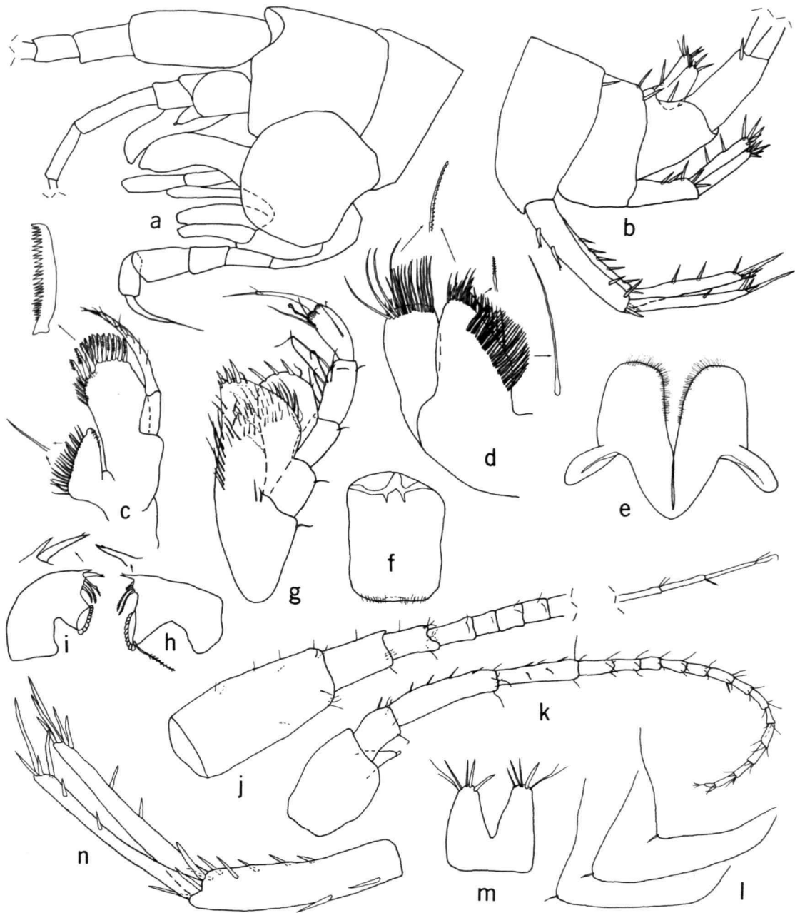
FIGURE 6.— Texiweckelia insolita , new species, paratype, artesian well, Hays County, Texas, female (4.5 mm): a, head region (setae and spines omitted); b, uronites with uropods 1 and 2, telson and uropod 3 in part; c, d, maxillae 1, 2 (setae and spines enlarged); e, lower lip; f, upper lip; g, maxilliped; h, right mandible (incisor enlarged); i, left mandible (incisor and lacinia mobilis enlarged); j, k, antennae 1, 2; l, pleonal plates; m, telson; n, uropod 1. (All mouthparts to same scale; head and uronites to same scale.)
