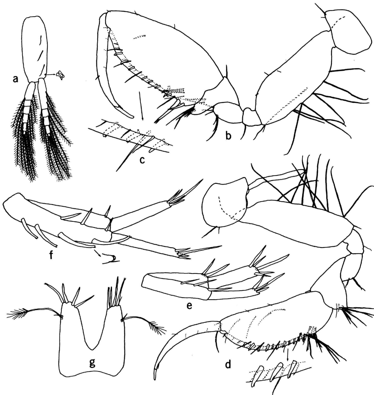
FIGURE 21.— Artesia subterranea , new species, paratype, artesian well, Hays County, Texas, female (5.5 mm): a, pleopod 3 (coupling spines enlarged); b, gnathopod 1 (lateral view); c, medial view of part of palm (enlarged); d, gnathopod 2 (lateral view; spines enlarged); e, uropod 2. Male (5.0 mm); f, uropod 1 (apex of spine enlarged); g, telson.
