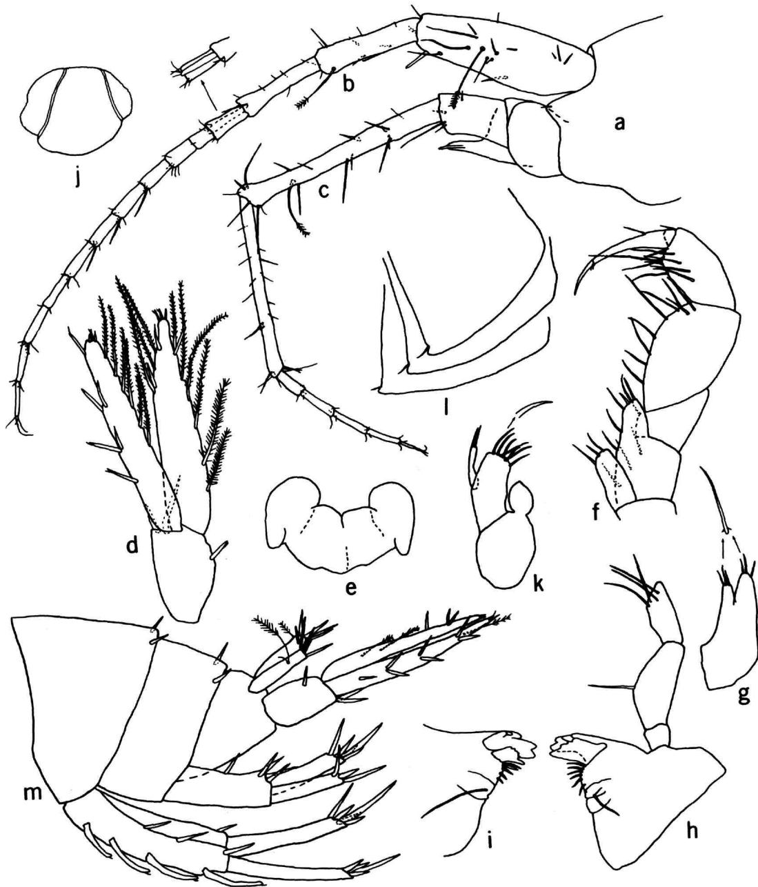
FIGURE 20.— Artesia subterranea , new species, paratypes, artesian well, Hays County, Texas, female (5.5 mm): a , head; b , c , antennae 1, 2 (head and antennae shown intact, medial view of accessory flagellum also shown); d , uropod 3; e , lower lip; f , maxilliped; g , maxilla 2 (setae enlarged); h , right mandible; i , dentate part of left mandible. Male (5.0 mm): j , upper lip; k , maxilla 1 (spine enlarged); l , pleonal plates. Male (6.6 mm): m , uronites with uropods and telson (some setae omitted from uropod 3). (All mouthparts of both sexes to same scale.)
