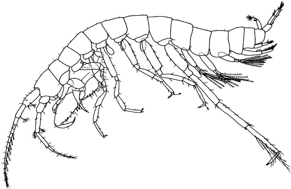
FIGURE 16.— Parabogidiella americana , new species, artesian well, Hays County, Texas, male (?) paratype (3.5 mm).
