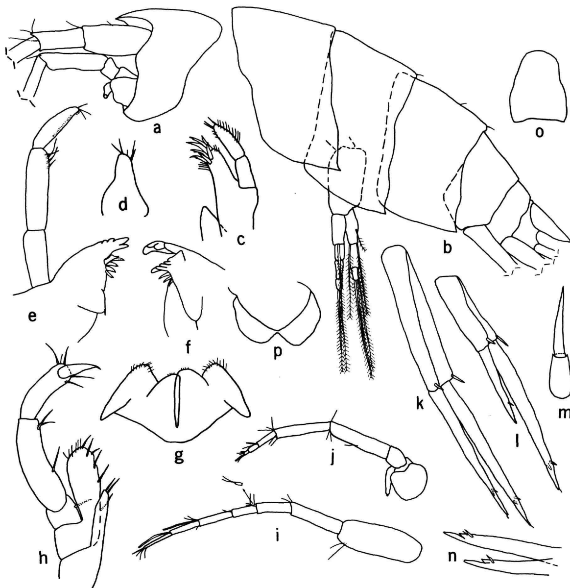
FIGURE 23.— Seborgia relictus , new species, paratypes, artesian well, Hays County, Texas, male (1.3 mm): a , head; b , pleonites and uronites with pleopod 2 and telson shown intact. Female (1.9 mm): c , d , maxillae 1, 2; e , left mandible; f , dentate part of right mandible; g , lower lip; h , maxilliped; i , j , antennae 1, 2; k , l , m , uropods 1, 2, 3. Male (1.3 mm): n , medial view of rami of uropod 1. Female (1.5 mm): o , telson; p , upper lip. (All mouthparts to same scale; head, pleonites, and uronites to same scale.)
