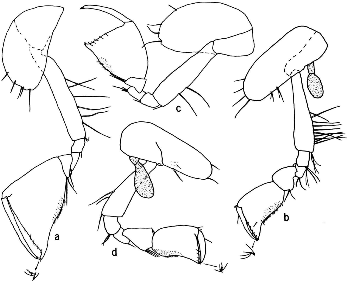
FIGURE 24.— Seborgia relictus , new species, paratypes, artesian well, Hays County, Texas, female (1.9 mm): a, b, gnathopods 1, 2 (lateral view). Male (1.5 mm): c, d, gnathopods 1, 2 (medial view). (Tip of dactyls and defining angles enlarged.)
