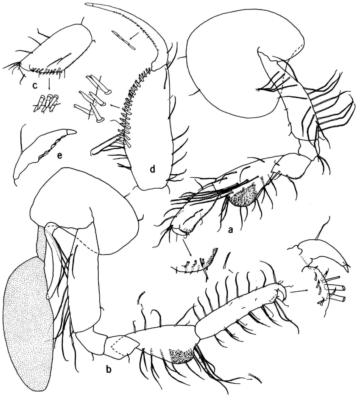
FIGURE 10.— Texiweckelia samacos , new species, paratypes, artesian well, Hays County, Texas, female (7.3 mm): a, b, gnathopods 1, 2 (palms enlarged). Male (7.0 mm): c, d, gnathopod propods 1, 2 (spines enlarged); e, dactyl of gnathopod 1 (enlarged). (Gnathopods of both sexes to same scale.)
