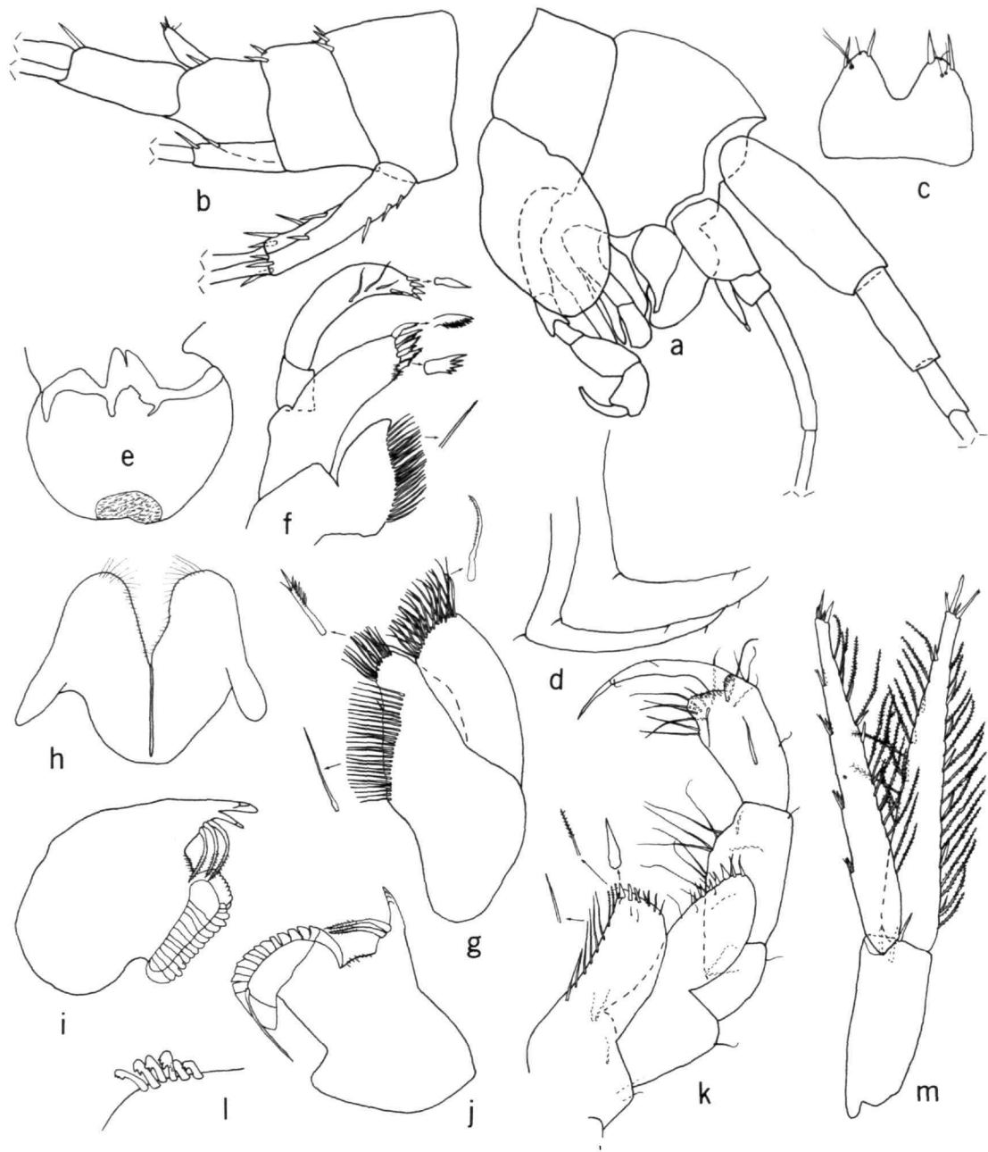
FIGURE 3.— Texiweckelia texensis (Holsinger), topotypes, artesian well, Hays County, Texas, male (6.0 mm): a, head region (setae and spines omitted); b, uronites with telson and uropods (in part). Female (6.0 mm): c, telson; d, pleonal plates; e, upper lip; f, g, maxillae 1, 2 (apical setae and spines enlarged); h, lower lip; i, left mandible; j, right mandible; k, maxilliped (setae and spines enlarged); l, coupling spines from peduncle of pleopod 2. Female (7.0 mm): m, uropod 3. (All mouthparts to same scale; head and uronites to same scale.)
