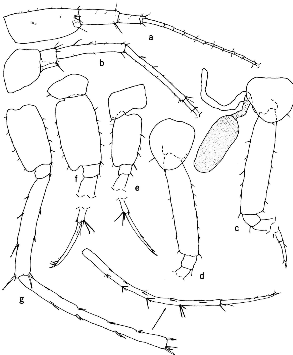
FIGURE 5.— Texiweckelia texensis (Holsinger), topotype, artesian well, Hays County, Texas, female (6.0 mm): a, b, antennae 1, 2; c, d, pereopods 3, 4 (in part); e, f, pereopods 5, 7 (in part); g, pereopod 6 (continuation of appendage indicated by arrow).
