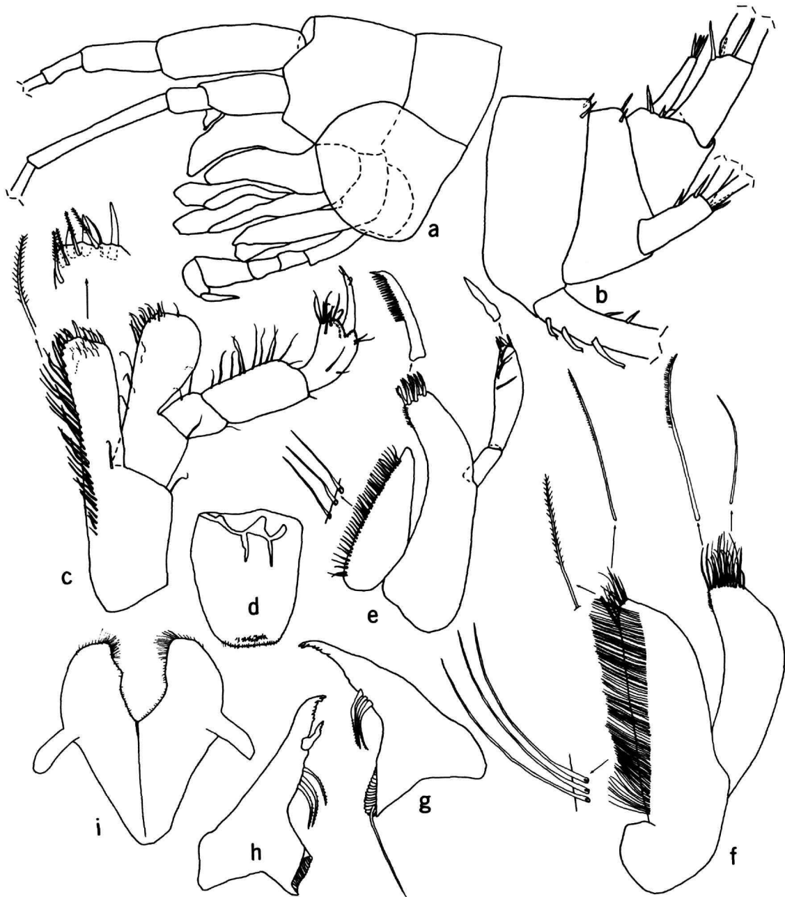
FIGURE 9.— Texiweckelia samacos , new species, paratypes, artesian well, Hays County, Texas, male (7.0 mm): a , head region (setae and spines omitted); b , uronites with telson and uropods (in part). Female (7.3 mm): c , maxilliped (setae and spines enlarged); d , upper lip; e , f , maxillae 1, 2 (setae and spines enlarged). Male 6.3 mm: g , h , right and left mandibles. Male (7.0 mm): i , lower lip. (Mouthparts to same scale except mandibles, which are at larger scale; head and uronites to same scale.)
