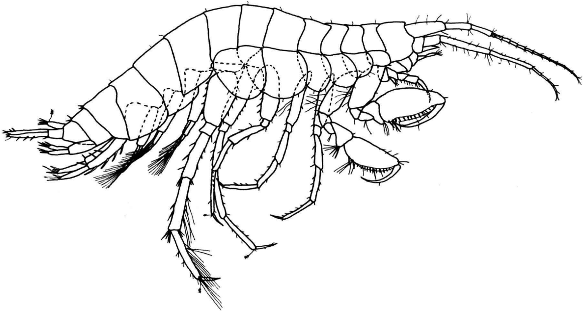
FIGURE 19.— Artesia subterranea , new species, artesian well, Hays County, Texas, female paratype (6.1 mm).
