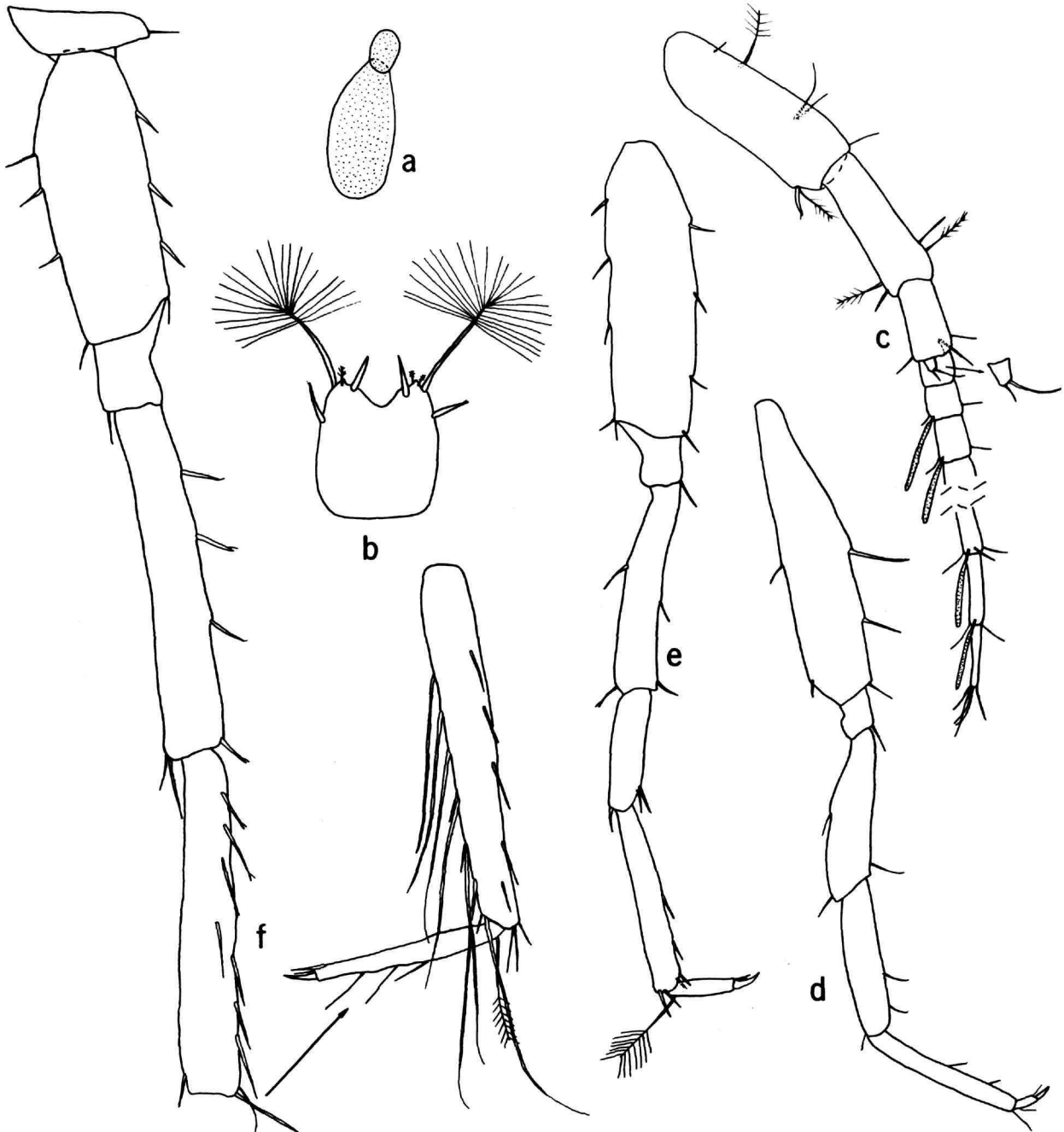
FIGURE 18.— Parabogidiella americana , new species, artesian well, Hays County, Texas, male (?) paratype (3.5 mm): a, coxal gill from pereopod 3; b, telson; c, antenna 1 (accessory flagellum enlarged); d, pereopod 3; e, f, pereopods 6, 7 (continuation of appendage indicated by arrow). (All pereopods to same scale.)
