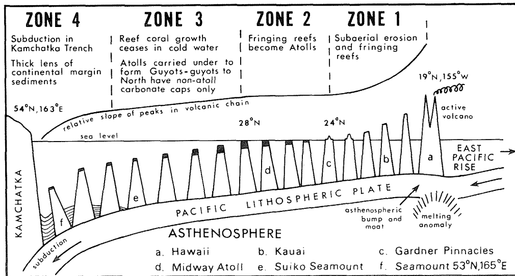
Figure 9. Schematic representation of the major physical factors influencing the Hawaiian-Emperor Seamount Chain (modified from Scott et al., 1976).
