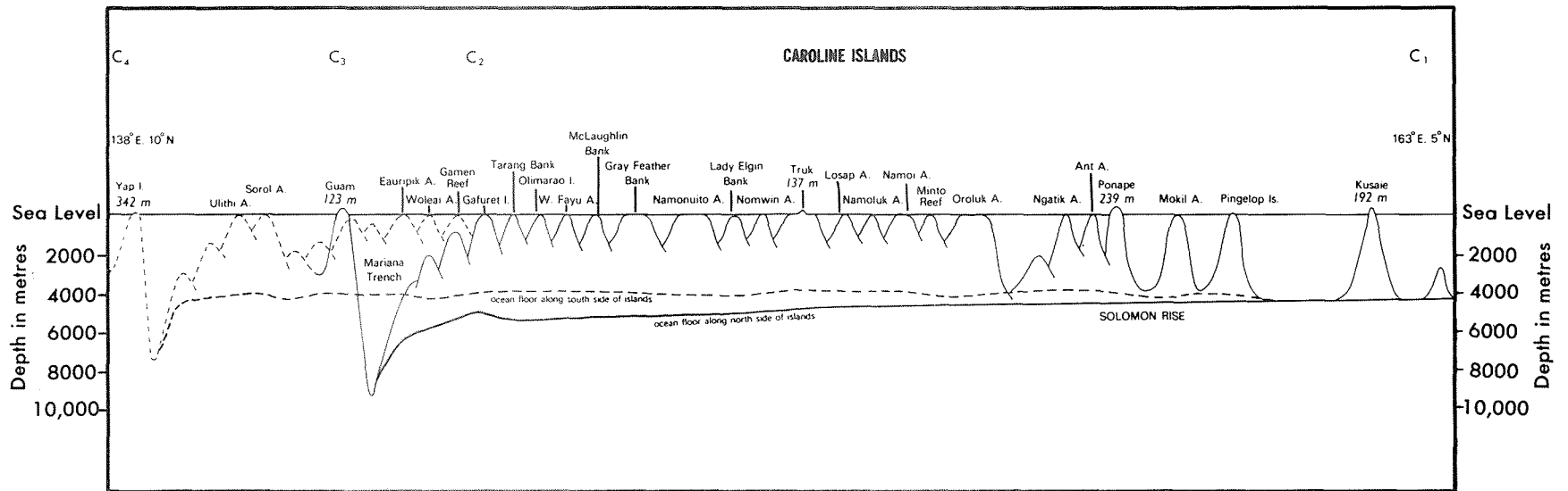
Figure 11. Profiles along the Caroline Island Chain.
