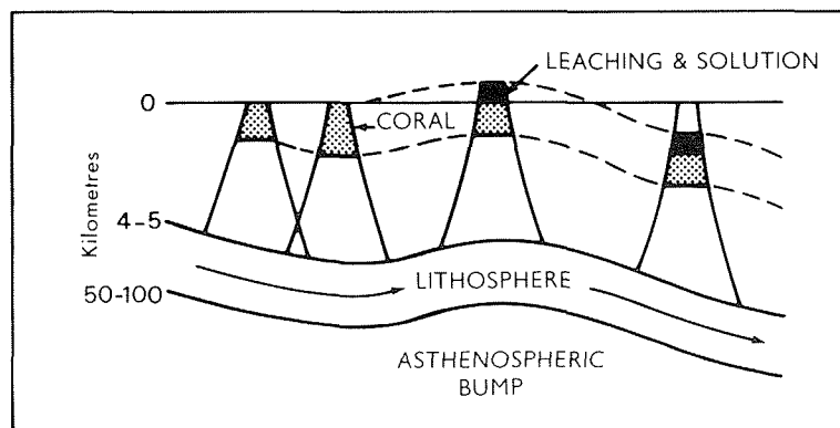
Figure 6. Idealized history of an atoll emerging-subsiding as it passes over an asthenospheric bump. After Menard (1973).
