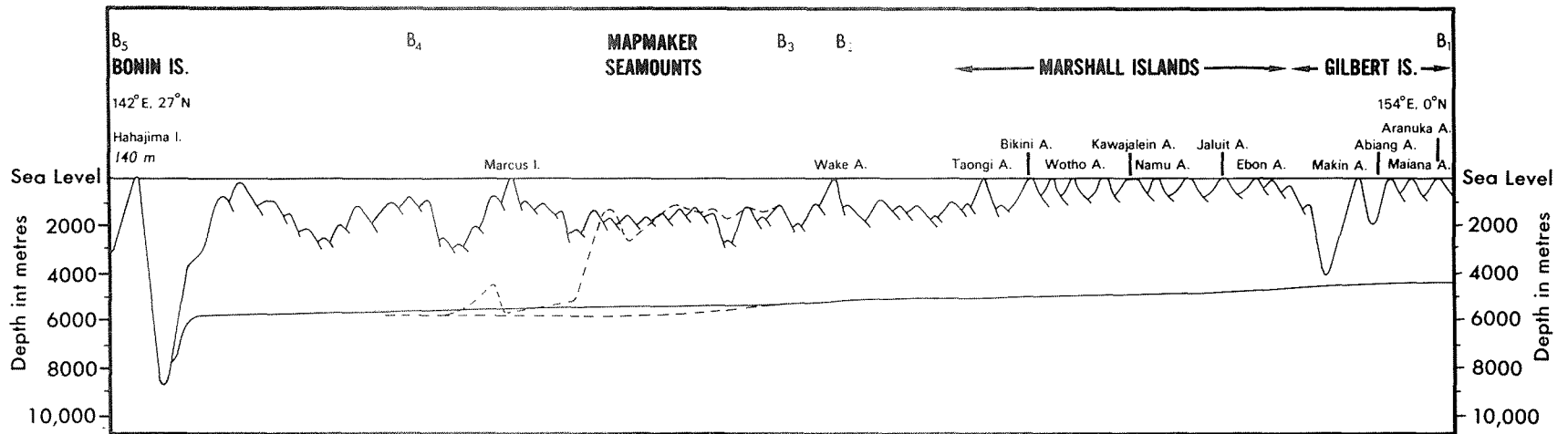
Figure 10. Profiles along the Marshall-Gilbert island chains.
