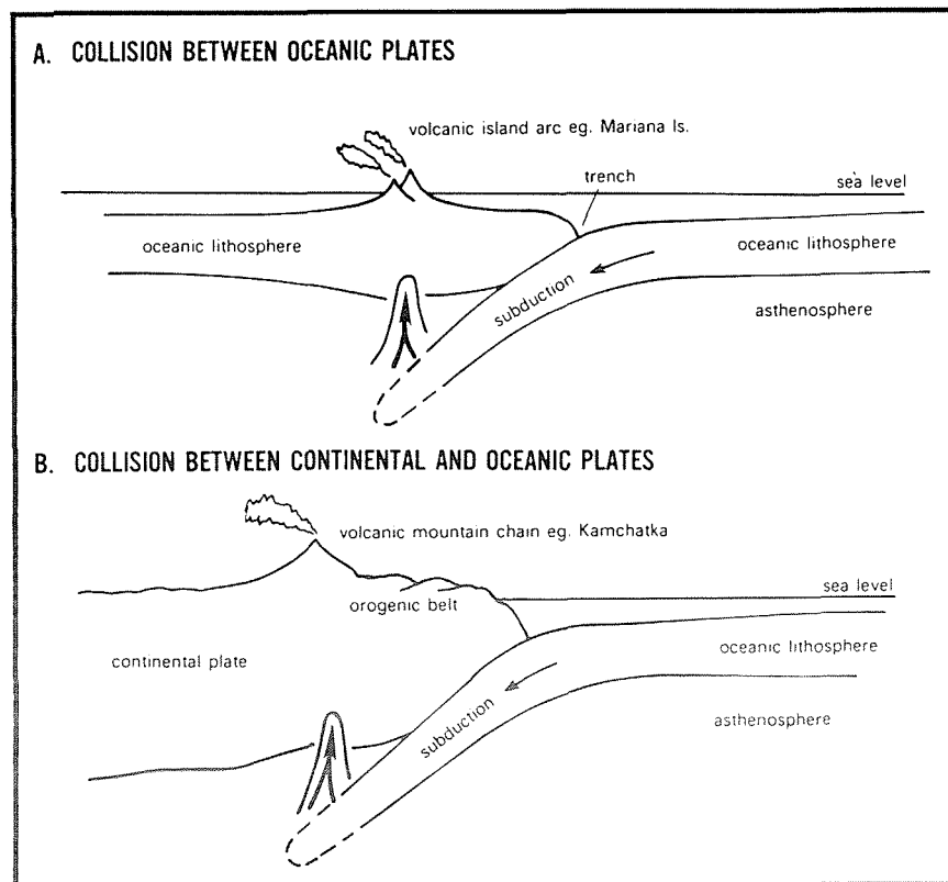
Figure 4. Typical subduction patterns in the western Pacific.
