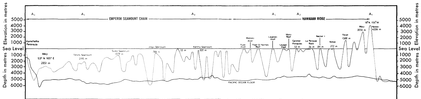
Figure 7. Profile of the Hawaiian-Emperor Chain (modified from Rotondo, 1975 Fig. 1.9). For profile route see Figure 2.
