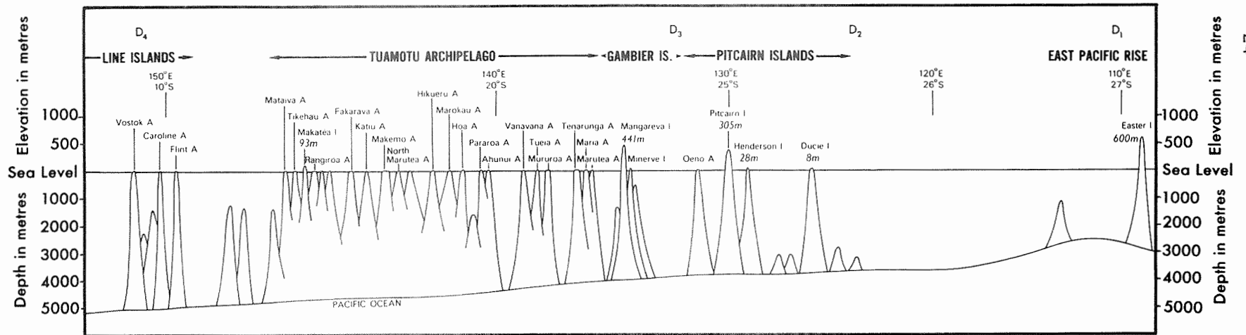
Figure 12. Profile from the East Pacific Rise through the Tuamotu Archipelago.
