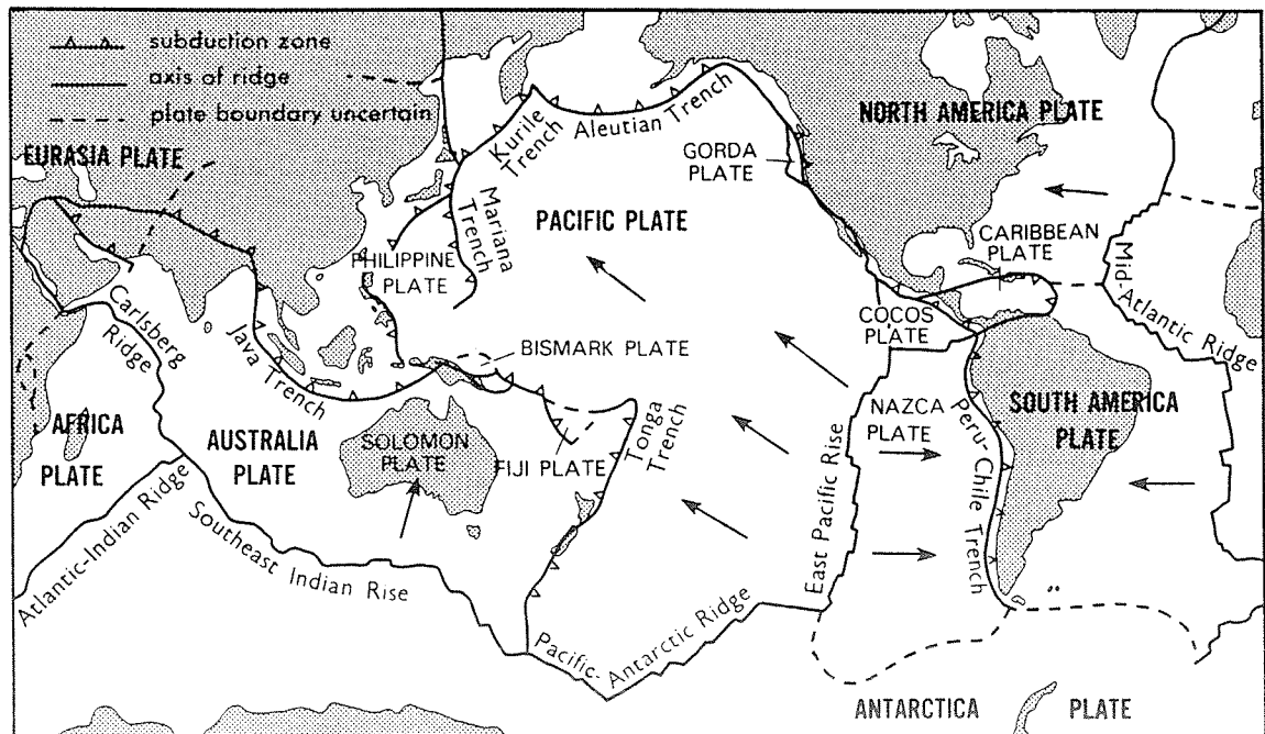
Figure 1. The Pacific lithospheric plate.
