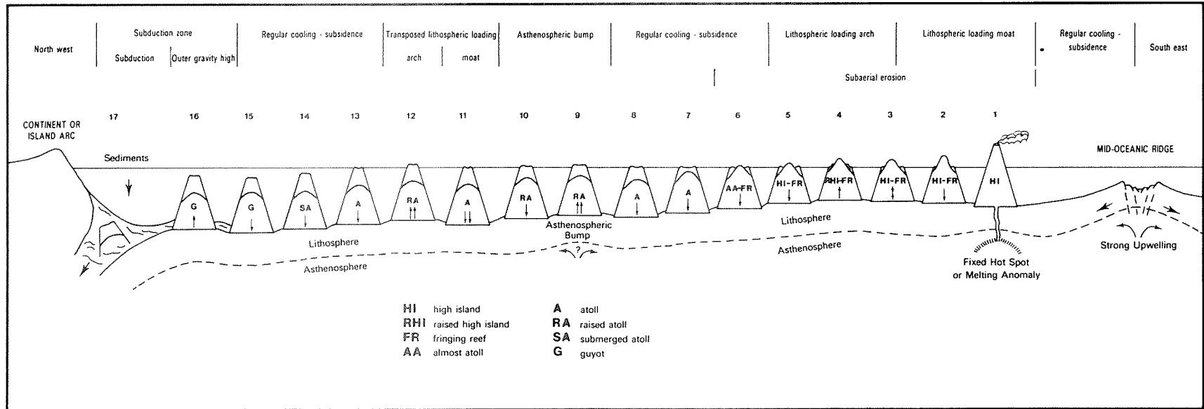
Figure 14. A model for island-type development on the Pacific lithosphere plate. For explanations of the seventeen positions indicated see text. Vertical arrows indicate relative rates of subsidence-emergence.
