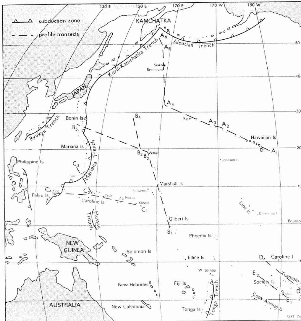
Figure 2. Western Pacific Ocean showing the major island groups mentioned in the text. Profile transects along dashed lines are shown in Figures 7 and 10-13.
