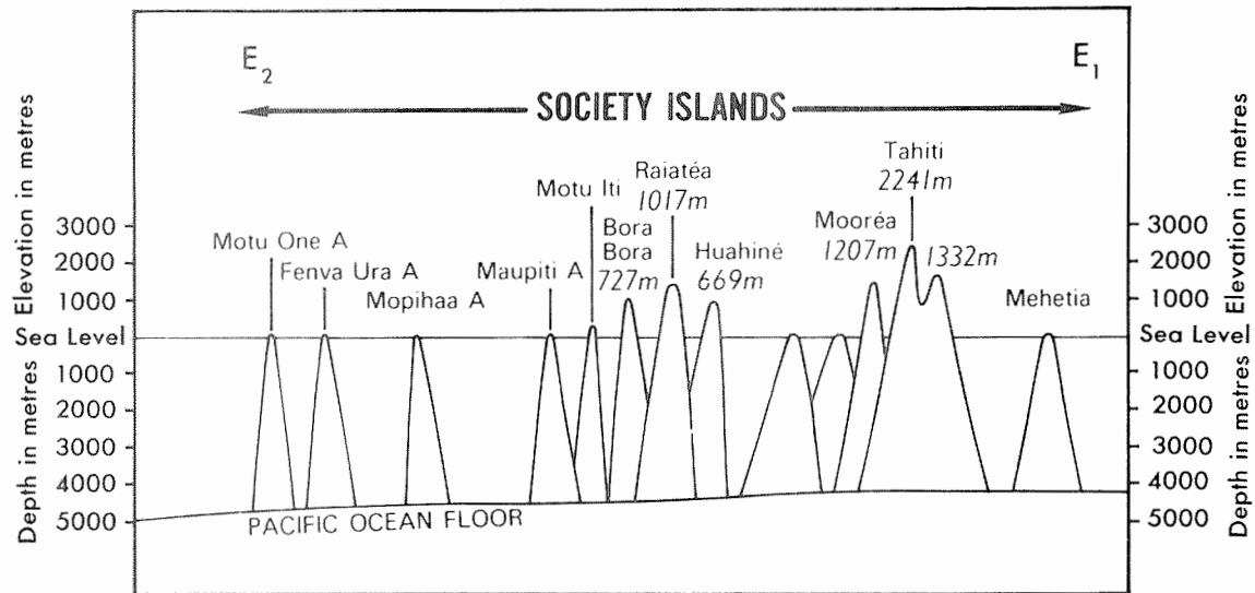
Figure 13. Profile through the Society Islands.
