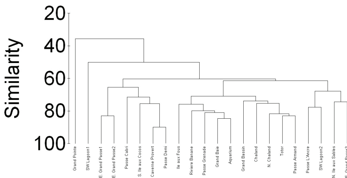
Fig. 4. Cluster analysis ( \sqrt{\text{transformed}} ) of the degree of coral bleaching at the 22 survey sites during March-April 2005.
