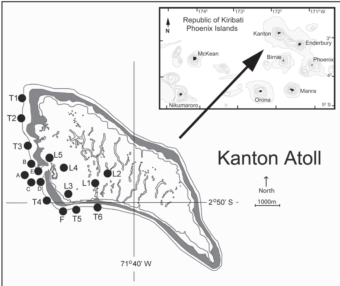
Figure 1. Location map for Kanton Atoll survey stations in the Phoenix Islands, Republic of Kiribati in the Central Pacific Ocean visited by the crew of the RV Heraclitus, November 22 through December 19, 2004. Stations include (1) Offshore Transects: T1 – T6, (2) Offshore Observational Dives: A – F, and (3) Lagoon Snorkel/Health and Vitality Dives: L1 – L5
