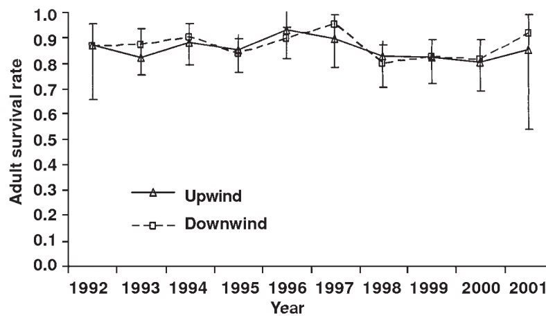
Fig. 3. Adult survival rates for birds upwind (triangle and solid line) and downwind (squares and dotted line) of the JACADS plant from 1992 to 2001 (Year t to t+1 ). Results are estimates and 95% confidence intervals from model \varphi_{site^t}^A \cdot \varphi_t^J \cdot \rho_{site^t} \cdot \psi_{site}^{age} \cdot \psi_{site^t}^{breeder} .
