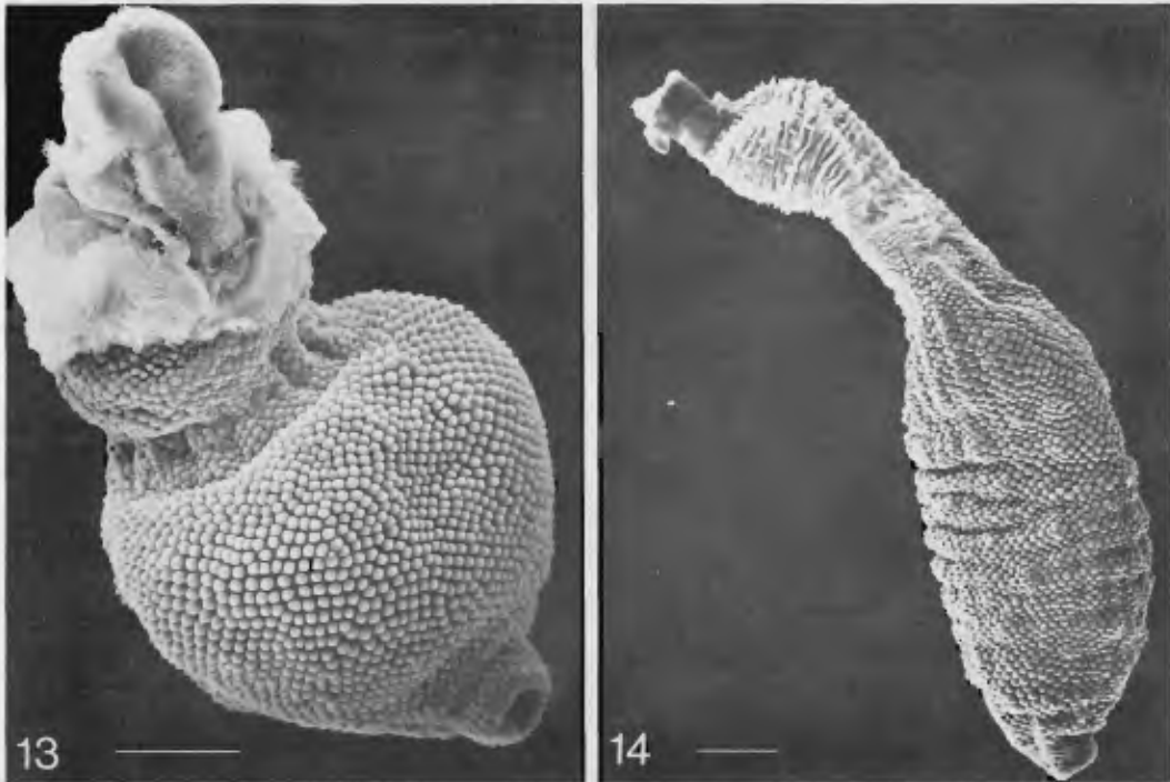
FIGS. 13-14. Scanning electron micrographs of planktotrophic pelagosphera larva and recently metamorphosed juvenile of Aspidosiphon sp. From
