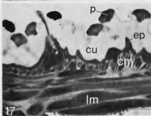
FIG. 15. Scanning electron micrograph of surface cuticular papillae of planktotrophic pelagosphaera from open-ocean plankton tentatively identified as belonging to the genus Phascolosoma . Scale, 2\ \mu\text{m} .
