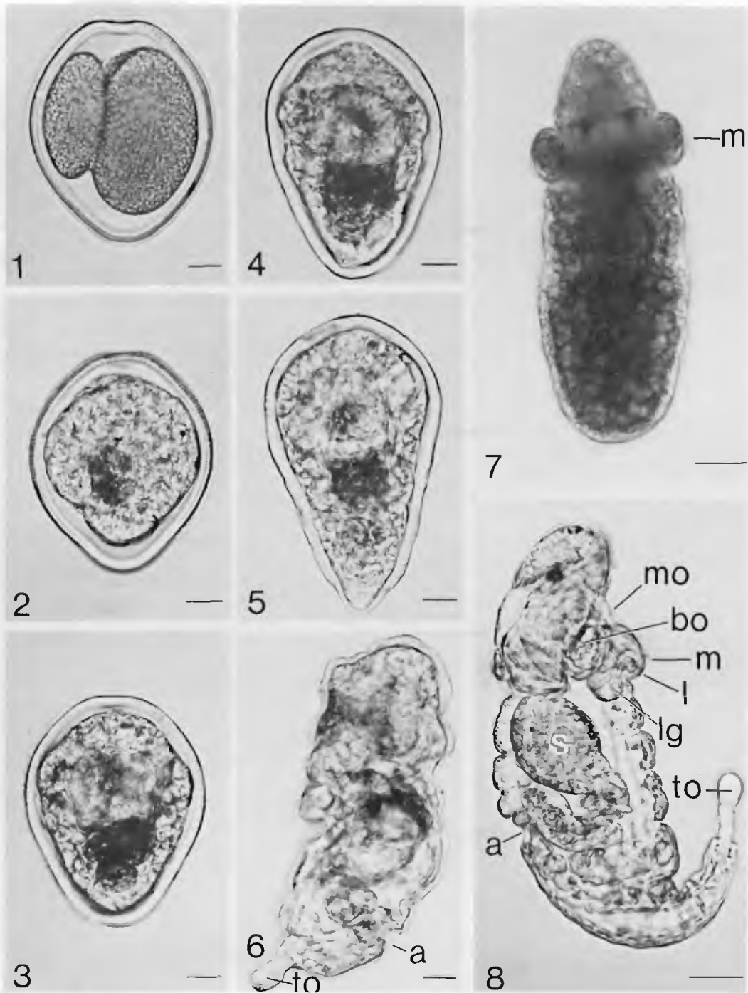
FIGS. 1-6. Developmental stages of Phascolosoma varians . Scale, 25 \mu m.
