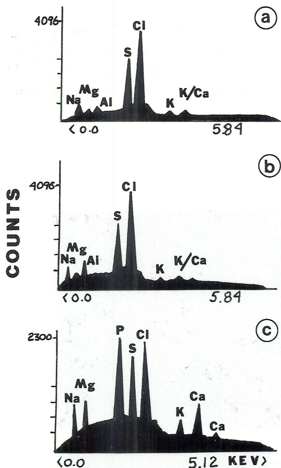
Fig. 4. Energy dispersive x-ray analysis: (a) Outer wall, (b) Inner wall. The presence of Al in (a) and (b) was shown to be an artifact of the instrumentation as wavelength dispersive x-ray analysis with an ARL SEM-Q failed to reveal any Al. (c) Nidimental gland secretions. The gland showed similar elemental composition to (a) and (b) with the exception of large amounts of P and higher amounts of Mg and Ca (see text for explanation).
