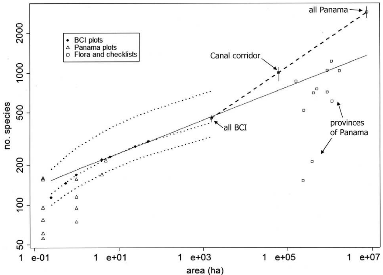
Fig. 3. Species-area relationship for trees and shrubs. The solid line gives the best fit power-function SAR for plots from 1 ha to 50 ha at Barro Colorado ( S=173\text{area}^{0.146} ). The dashed line is the fit to the three points indicated with arrows ( S=91\text{area}^{0.218} ). The dotted lines give predictions from Fisher's \alpha , with \alpha = 26, 35, and 60 , representing mean values for a from the Pacific region, Barro Colorado, and eastern wet forests.
