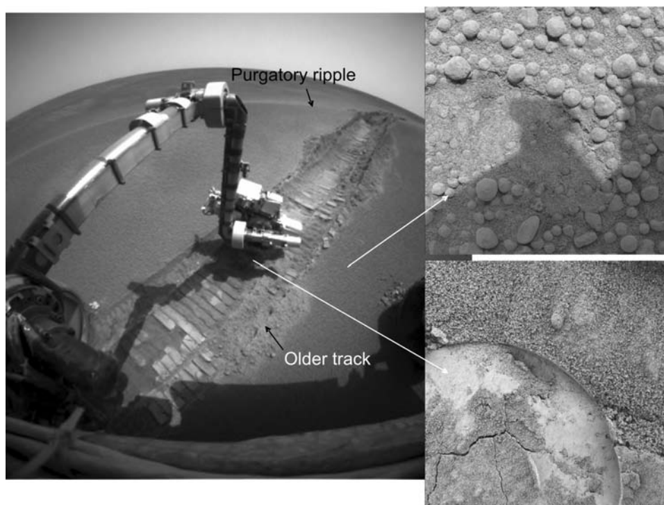
Figure 14. Hazcam and MI views of Purgatory ripple after Opportunity backed out. Very well defined molds are evident, consistent with a relatively high abundance of fine-grained materials. Ubiquitous hematitic concretions are still evident for the undisturbed surface. Older track where exposed is brighter than the younger track, probably because of dust deposition. Note the shadow of the IDD turret at the top of upper MI frame. Bottom MI frame was acquired while target was fully shadowed. Hazcam frame number is 1F173279793EDN55W4P1131L0M1; MI frames acquired on sol 507 are (top) 1M173191578EFF55W4P2956M2F1 and (bottom) 1M173193890EFF55W4P2936M2F1. MI images cover \sim 3 cm in width and height.
