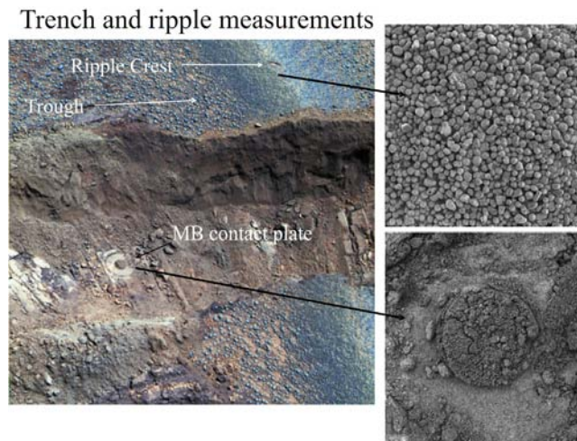
Figure 11. Pancam and MI views of the sol 366 trench and areas analyzed using IDD instruments. Ripple crest is densely covered by hematitic concretions whereas the trough is covered by a less dense array of larger hematitic concretions, with bright red and dark substrate exposed. The steep trench wall, clods, and the mold due to placement of the MB contact plate imply that the exposed soil is slightly coherent and poorly sorted. MI images show sand and finer-grained materials are present. Pancam frames acquired on sol 372 are: 1P161207836EFF42DIP2374L2C1, 1P161207869EFF42DIP2374L5C1, 1P161207895EFF42DIP2374L7C1. MI frames acquired on sol 368 are: (top) 1M160851916EFF42D9P2997M2F1 and (bottom) 1M160851441EFF42D9P2997M2F1, both acquired when the targets were fully shadowed. MI images cover \sim 3 cm in width and height.
