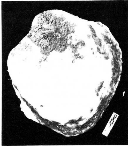
Fig. 2. Dorsal valve of Ostrea edulis L. (USNM 836258) from the carapace of a nesting female Caretta caretta (L.) on Zakynthos Island, Greece; note: thick cover of filamentous algae and deep scratches in shell.
