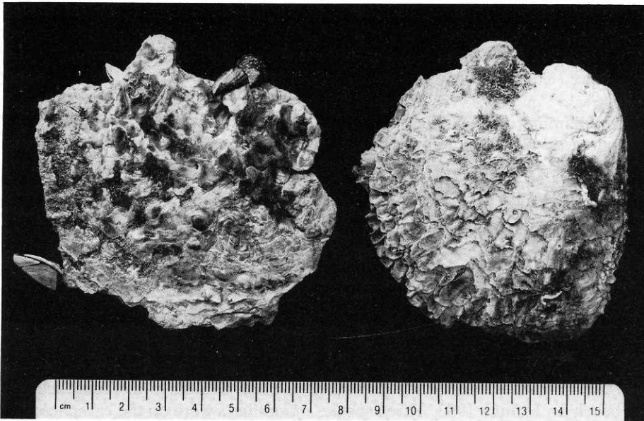
Fig. 4. Ventral (left) and dorsal (right) valves of Ostrea edulis L. (USMN 804417) from a nesting female Caretta caretta (L.) on Peloponnesus, Greece; note: Lepas hillii LEACH and Mytilus edulis L. attached to ventral valve and algae and worm tubes on dorsal valve.
