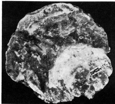
Fig. 1. Ventral valve of Ostrea edulis L. (USNM 836256) from the carapace of a nesting female Caretta caretta (L.) on Zakynthos Island, Greece; note: parts of three scales, divided by three radiating lines, left by the removal of parts of the keratinous scales of the turtle's carapace.
