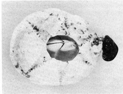
Fig. 3. Chelonibia sp. (USNM 211342) with a Mytilus edulis L. attached to it; the barnacle, 43 mm in diameter, was attached to the same nesting female Caretta caretta (L.) from Zakynthos Island, Greece which carried the Ostrea edulis L. illustrated in Fig. 2.
