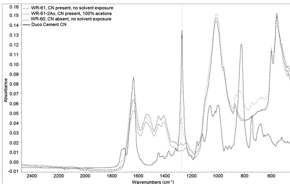
Fig. 1 FTIR spectra showing the removal of cellulose nitrate (CN) from bone samples. The presence of CN in bone samples is indicated by the absorption band (symmetric \text{NO}_2 stretch) at 1274 \text{ cm}^{-1} . The figure shows spectra from Duco cement reference sample (solid line), control bone
