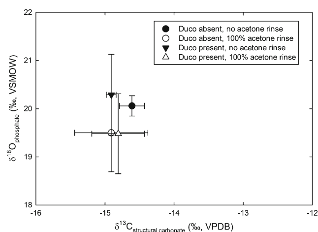
Fig. 3 Average phosphate oxygen isotope values (plotted against structural carbonate carbon values for comparison) for whale rib samples according to sample treatment. Error bars represent 1\sigma standard deviation of replicate analyses
