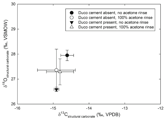
Fig. 4 Average structural carbonate oxygen and carbon isotope values for whale rib samples according to sample treatment. Error bars represent 1 \sigma standard deviation of replicate analyses
