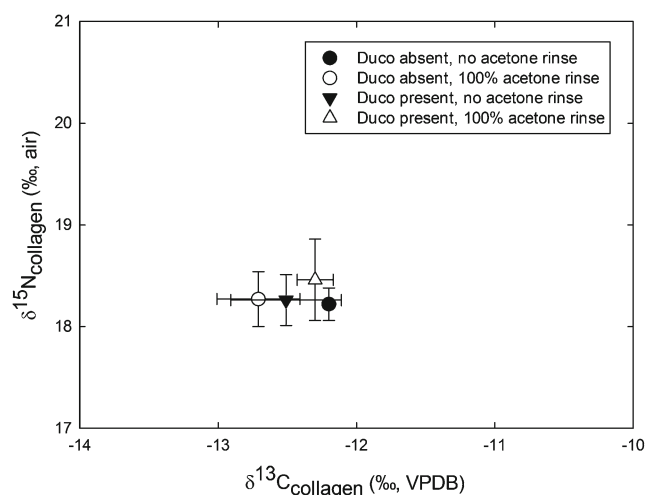
Fig. 2 Average collagen carbon and nitrogen isotope values for seal femur samples according to treatment categories. Error bars represent 1\sigma standard deviation of replicate analyses
