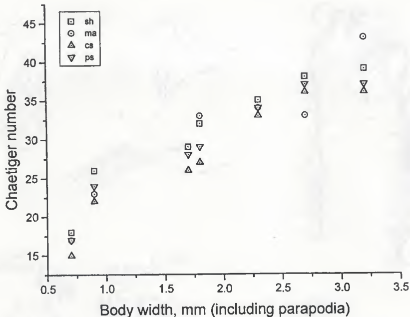
FIG. 21. The relationships between maximum body width (mm) and various chaetae positions in Euniphysa quadridentata n. sp. ( n=7 ): sh=start position of subacicular hook, ma=last chaetiger with multiple acicula, cs=start position of compound spiniger, ps=ending position of pseudocompound spiniger.
