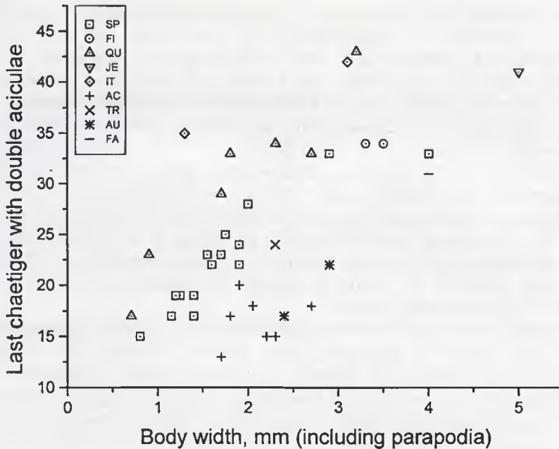
FIG. 7. The relationships between maximum body width (mm) and the ending position of multiple aciculae in nine Euniphysa species. Abbreviations as in figure 4.
