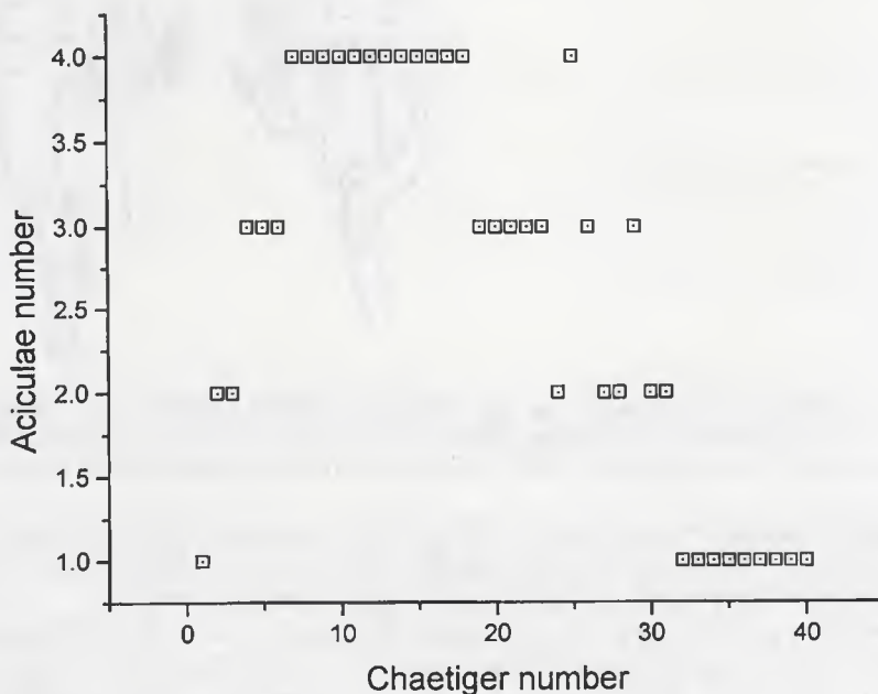
FIG. 20. The distribution pattern of aciculae in the anterior 40 chaetigers of Euniphysa quadridentata n. sp. (USNM 090047).
