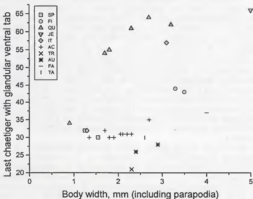
FIG. 5. The relationships between maximum body width (mm) and the ending position of ventral glandular tabs in 10 Euniphysa species. Abbreviations as in figure 4, TA = E. taiwanensis ( n=1 ).
