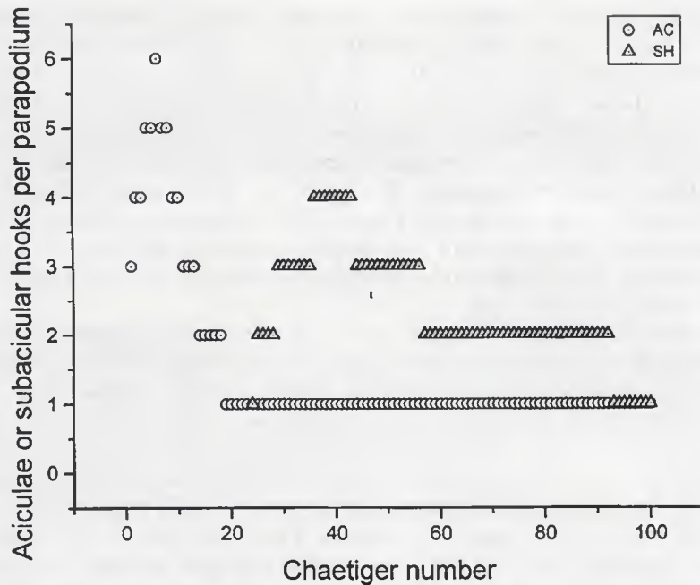
FIG. 11. The distribution pattern of aciculae and subacicular hooks in the anterior 100 chaetigers of the complete specimen of Euniphysa aculeata (USNM 96436). AC = aciculae; SH = subacicular hooks.
