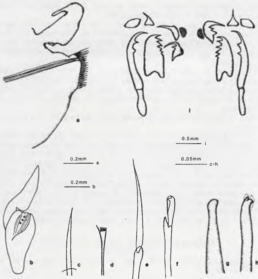
FIG. 23. Eunice tridontesa (paratype, SSBT-0031). (a) Parapodium 5; (b) parapodium 4, lateral view; (c) simple chaetae; (d) pectinate chaetae; (e) compound spiniger; (f) compound falciger; (g) acicula; (h) subacicular hook; (i) maxillae.
