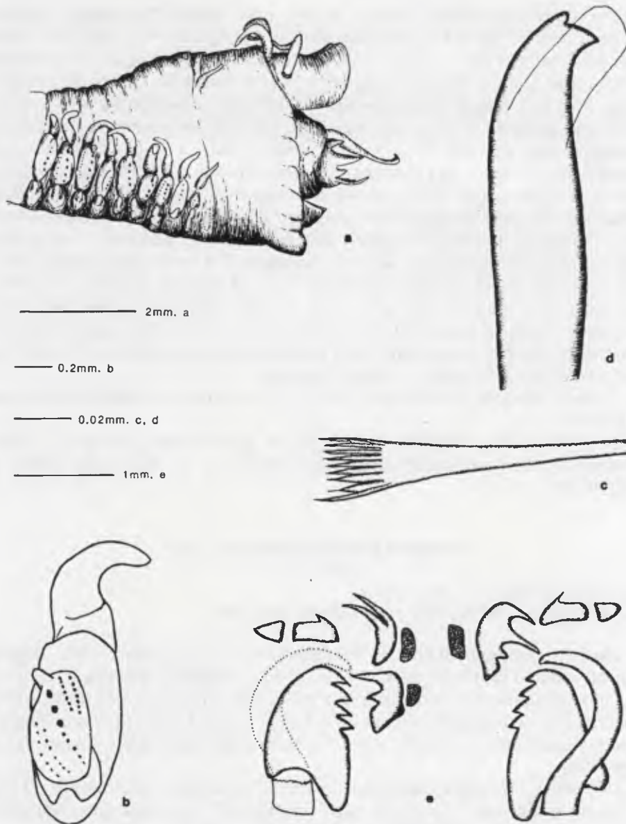
FIG. 18. Euniphysa jeffreysii (holotype, BM ZK 1921, 5.1.1986). (a) Anterior end, lateral view; (b) parapodium 4, lateral view; (c) pectinate chaetae; (d) subacicular hook; (e) maxillae.
