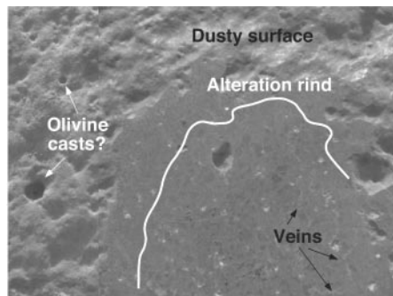
Fig. 2. Composite MI image (no. 2M131690279EFF1155P2939M2M1) of an oblique RAT grind into Humphrey, illustrating its natural surface containing hexagonal casts, a brushed surface, an inferred alteration rind, and an interior containing tiny, irregular veins. The view is \sim 3\text{ cm} wide.
