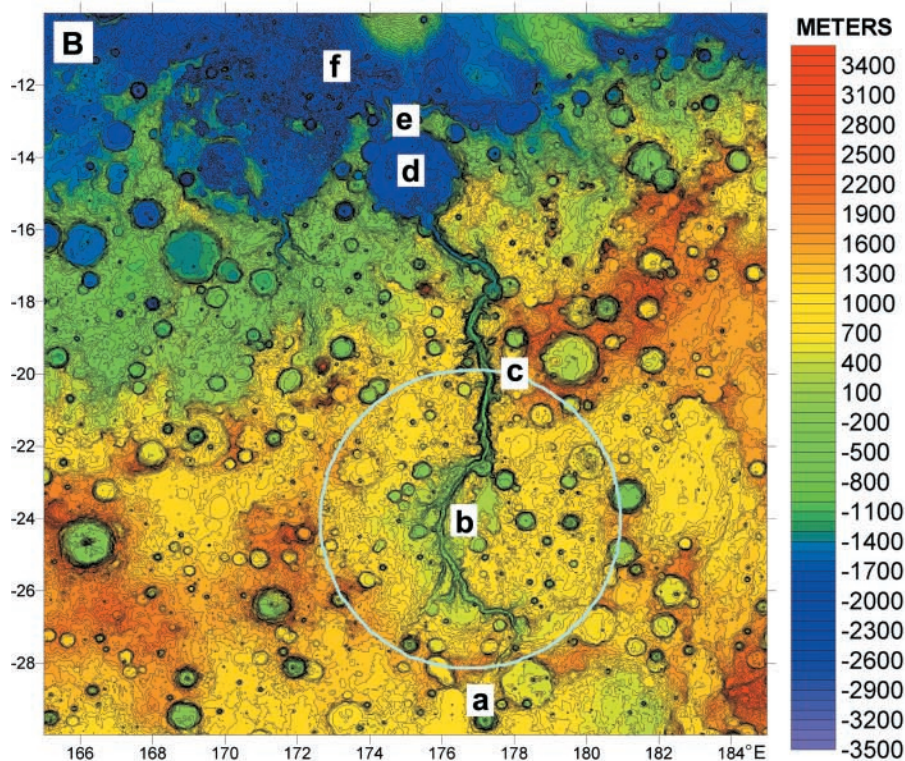
Fig. 1 (left). (A) Topography of lake sub-basins that overflowed to Ma'adim Vallis (a, b, and c) and isolated lake basins (d and e). The blue circle is the Ma'adim impact basin, and drainage divides (white lines) surround the lake's high stand at 1100 m (black line). (B) Topography of Ma'adim Vallis, showing the Ma'adim basin rim crosscut at (c) and at the valley head (a), dissected basin floor (b), Gusev crater (d), its exit breach (e), and undissected lowlands (f). Both figures are MOLA topography (cylindrical projection, 100-m interval).
