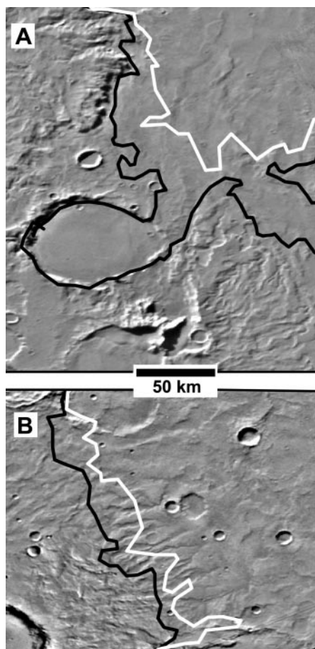
Fig. 3. Shoreline morphology in the lake basin, from Viking 256 pixel/degree mosaics. Valley networks either stop abruptly [(A) centered at 43.75°S, 184.5°E] near the black 1100-m contour, the lake's likely high stand, or widen below that level [(B) centered at 37.5°S, 159°E] if slopes were available in the basin. The white line is the 950-m contour.
