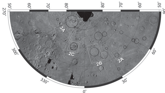
Figure 1. Mosaic of Mercury Dual Imaging System (MDIS) images of part of the high northern latitudes of Mercury. The region is dominated by volcanic smooth plains. Locations of buried impact craters and basins that contain graben enclosed by a wrinkle-ridge ring are indicated by black circles. Locations of Figures 2A, 2B, 2C, and 3A are also shown.
