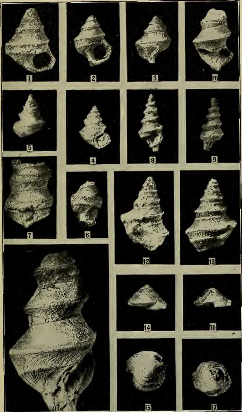
KANGYAO FORMATION
