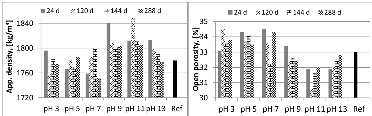
Figure 6. Left: Apparent density ( \text{kg/m}^3 ), average standard deviation \pm 18 . Right: % Open porosity, average standard deviation \pm 1 .
