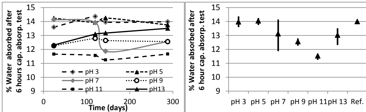
Figure 5. Left: Amount of water absorbed by capillarity after 6 hours of CA test at the various pH. The most regular patterns are obtained at pH 9 and 11. Right: Maximum, minimum and average values obtained at the various pH and for the reference.
