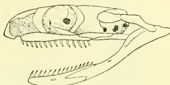
Fig. 4. PROFILE OF SKULL OF LAMPROPVELTIS (After Jan.)
