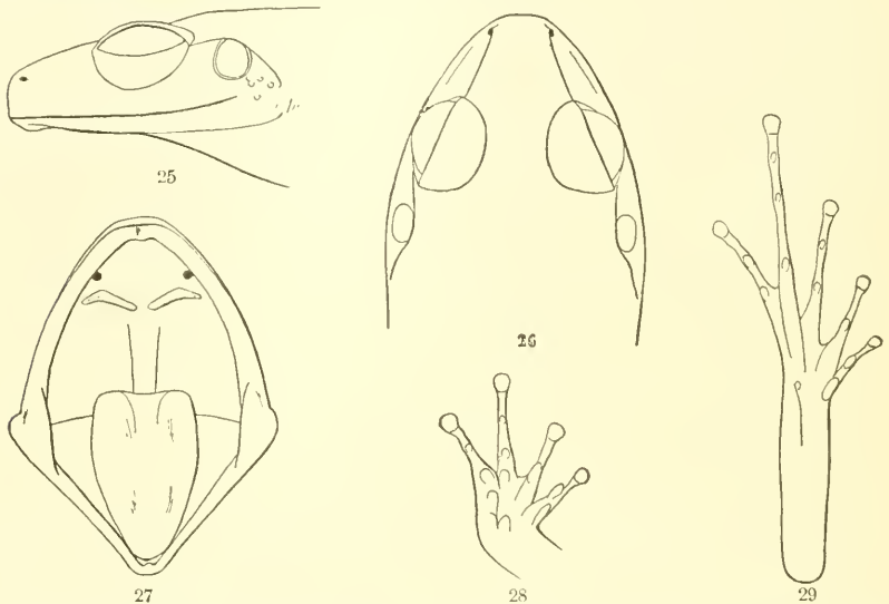
FIGS. 25-29.—ELEUTHERODACTYLUS RICHMONDI. 2 × natural size. 25, side of head; 26, top of head; 27, inside of mouth; 28, underside of fore foot; 29, underside of hind foot. No. 26884, U.S.N.M.
