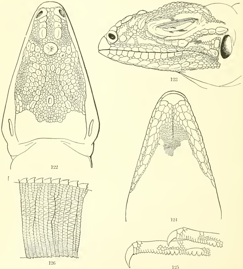
FIGS. 122-126.— CYCLURA CORNUTA . 1\frac{1}{2} \times natural size. 122, top of head; 123, side of head; 124, under-side of head; 125, toes, showing "comb;" 126, scales on side of tail. No. 23667, U.S.N.M.
