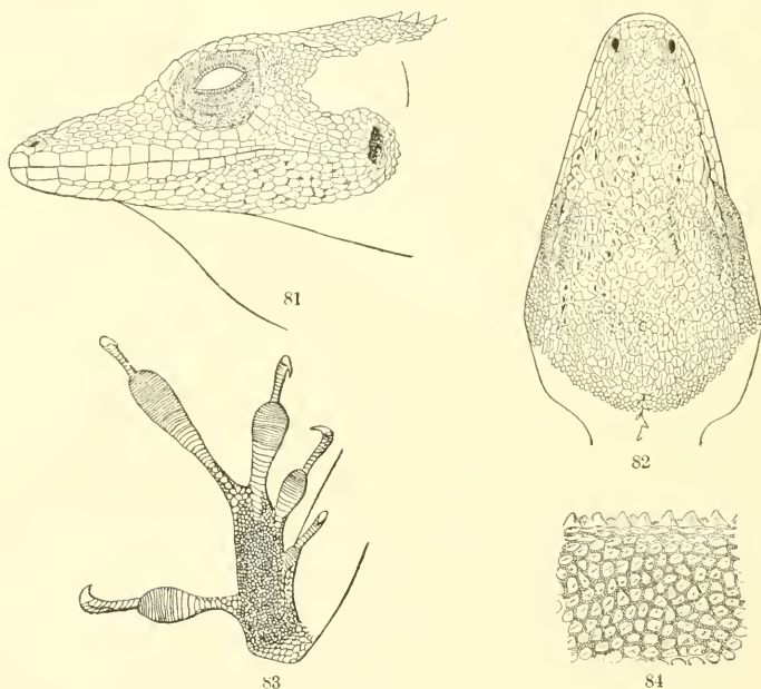
FIGS. 81-84.— ANOLIS CURVIERI . 81, side of head; 82, top of head; 83, under side of hind foot. Nat. size. 84, skin on side of neck, and dorsal crest. 2\times natural size. No. 26999, U.S.N.M.
