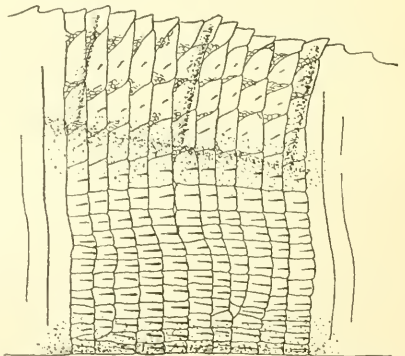
FIG. 88.— ANOLIS RICORDII . Santo Domingo. Side of tail at level of fifth spine. 2\times natural size. No. 12108, U.S.N.M.
