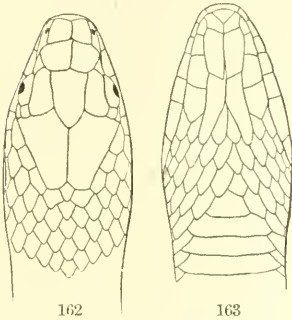
FIGS. 162-163.—LEIMADOPHIS STAHLI. 2\times natural size. 162, top of head; 163, underside of head. No. 26883, U.S.N.M.
