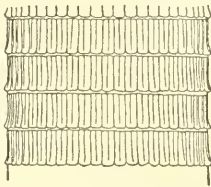
FIG. 66.— AMEIVA EXUL . 2× natural size. Dorsal view of portion of tail. No. 27221, U.S.N.M.
