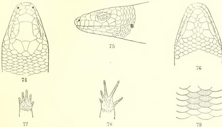
FIGS. 74-79.— CELESTUS PLEIL . 74, top of head; 75, side of head; 76, underside of head; 77, underside of right fore foot; 78, underside of left hind foot. 2\times natural size. 79, scales on back, showing arrangement and striation. 4\times natural size. No. 27066, U.S.N.M.
