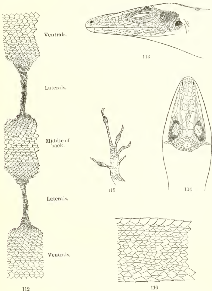
FIGS. 112-116.— ANOLIS PULCHELLUS . 112, scales around middle of body. 5\frac{1}{2} \times natural size. 113, side of head; 114, top of head. 2\frac{1}{2} \times natural size. 115, underside of hind foot. 2 \times natural size. 116, side of tail at level of fifth verticil. 5\frac{1}{2} \times natural size. No. 26799, U.S.N.M.
