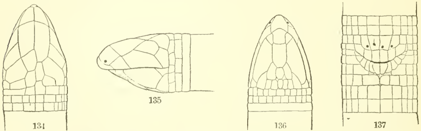
FIGS. 134-137.— AMPHIBLENA BAKERI . 2\frac{1}{2} \times natural size. 134, top of head; 135, side of head; 136, under-side of head; 137, anal region. No. 25537, U. S. N. M.
