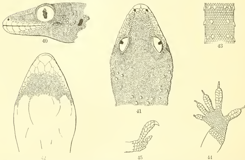
FIGS. 40-45.—HEMIDACTYLUS MABOUIA. 40, side of head; 41, top of head; 42, underside of head; 43, portion of upper surface of tail; 44, underside of hind foot. 2 \times natural size. 45, lateral view of last joint of toe. 4 \times natural size. No. 27630, U.S.N.M.
