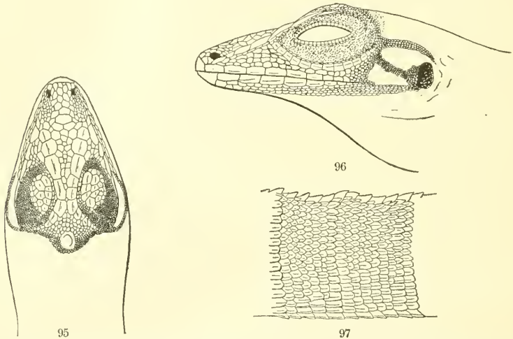
FIGS. 95-97.—ANOLIS CRISTATELLUS. Culebra Island. 95, top of head; 96, side head. 2\frac{3}{4} \times natural size. 97, side of tail at level of fifth vertebra. 5\frac{1}{4} \times natural size. No. 25777, U.S.N.M.
