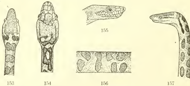
FIGS. 153-157.—EPICRATES MONENSIS, young. 153, color pattern, top of head; 154, color pattern, top of head of another specimen; 155, side of head, scutellation; 156, color pattern of body, lateral view; 157, color pattern, side of head and neck. Copies from Zenneck, figs. 53-62. Specimens in Hamburg Museum.
