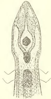
FIG. 52.—SPHÆRODUCTYLUS GRANDISQUAMIS. 2\frac{3}{4} in. natural size. Color pattern of head and shoulder. No. 27312. U.S.N.M.
