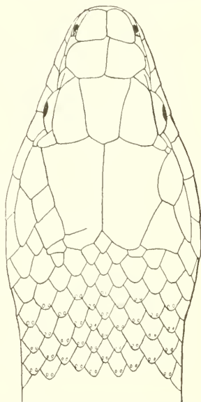
FIG. 170.— ALSOPHIS PORTORICENSIS . 2 × natural size. No. 27766, U.S.N.M.
