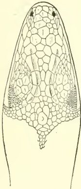
FIG. 121.—ANOLIS PONCENSIS. Top of head. 4 × natural size. No. 27290, U.S.N.M.
