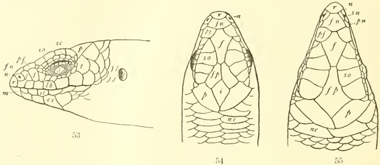
FIGS. 53-55.—HEAD-SHIELDS OF SCINCID LIZARD. cs , Chin-shields; d , disk on lower eyelid; c , ear-opening; f , frontal; fn , frontonasal; fp , frontoparietal; i , interparietal; lb , lower labials; m , mental; n , nasal; nc , nuchals; p , parietals; pf , prefrontal; pn , postnasal; r , rostral; sc , supraciliaries; sn , supranasal; so , supraocular; t , temporal.
