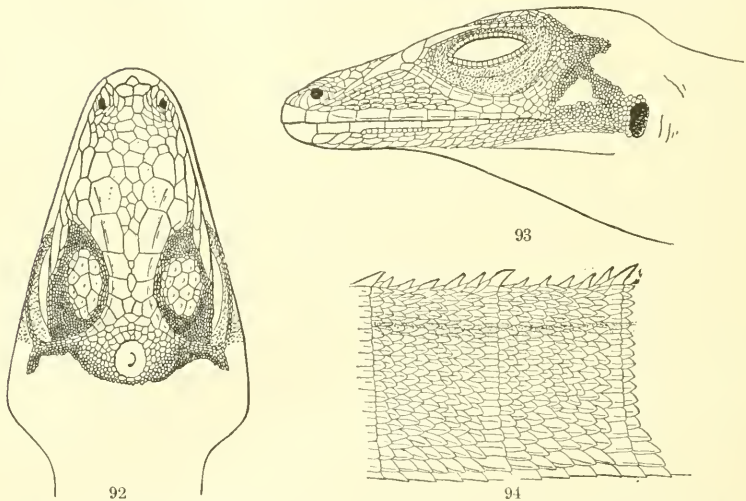
FIGS. 92-94.—ANOLIS CRISTATELLUS. 92, top of head; 93, side of head. 2\frac{1}{2} \times natural size. 94, side of tail at level of fifth spine. 5\frac{1}{2} \times natural size. No. 26803, U.S.N.M.
