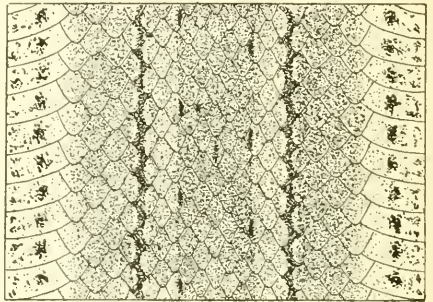
FIG. 164.—LEIMADOPHIS STAHLI. 2\times natural size. Color pattern around middle of body. No. 26883, U.S.N.M.
