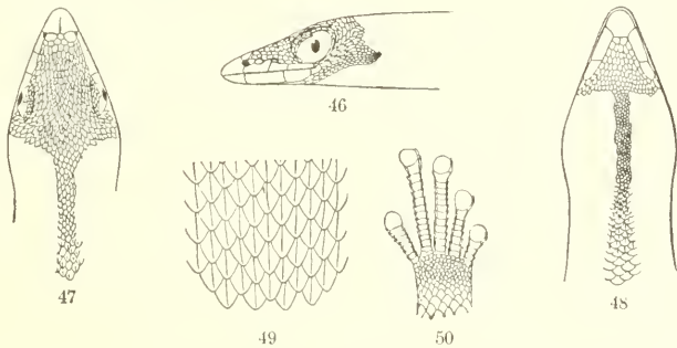
FIGS. 46-50.—SPHÆRODACTYLUS GRANDISQUAMIS. 46, side of head; 47, top of head; 48, underside of head. 2\frac{1}{2} \times natural size. 49, scales on middle of back; 50, underside of hind foot. 4 \times natural size. No. 27007, U.S.N.M.
