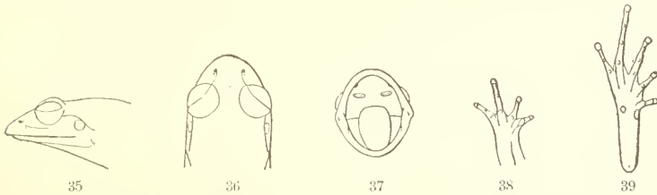
FIGS. 35-39.—ELEUTHERODACTYLUS UNICOLOR. 35, side of head; 36, top of head; 37, inside of mouth; 2 \times natural size. 38, underside of fore foot; 39, underside of hind foot. 2 \times natural size. No. 26963, U.S.N.M.
