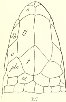
FIGS. 127-128.—SHIELDS ON HEAD OF AMPHISBÆNA. f , frontal; lb , supralabial; 1lb , first supralabial; 2lb , second supralabial; 3lb , third supralabial; 2ll , second lower labial; m , mental; mal , malar; n , nasal; o , ocular; oc , occipital; pf , prefrontal; pm , postmental; pto , postocular; r , rostral; t , temporal.
