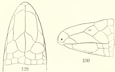
FIGS. 129-130.— AMPHISBENA CAECA . \frac{3}{4} natural size. 129, top of head; 130, side of head. No. 27223, U.S.N.M.
