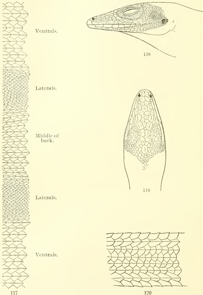
FIGS. 117-120.— ANOLIS PONCENSIS . 117, scales around middle of body. 5\frac{1}{2} \times natural size. 118, side of head; 119, top of head. 2\frac{2}{3} \times natural size. 120, side of tail at level of fifth vertebra. 5\frac{1}{2} \times natural size. No. 27294, U.S.N.M.
