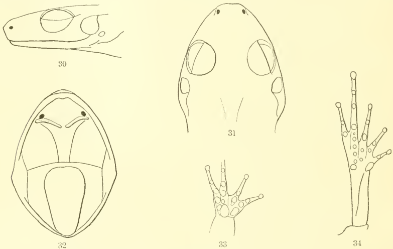
FIGS. 30-34.—ELEUTHERODACTYLUS MONENSIS. 2 . . natural size. 30, side of head; 31, top of head; 32, inside of mouth; 33, underside of fore foot; 34, underside of hind foot. No. 29389, U.S.N.M.
