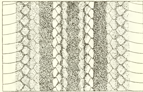
FIG. 166.—LEIMADOPHIS PARVIFRONS. Haiti. 2× natural size. Color pattern around the middle of the body. No. 9831, U.S.N.M.
