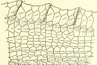
FIG. 87.— ANOLIS CUVIERI . Side of tail at level of fifth spine. 2\times natural size. No. 26843, U.S.N.M.
