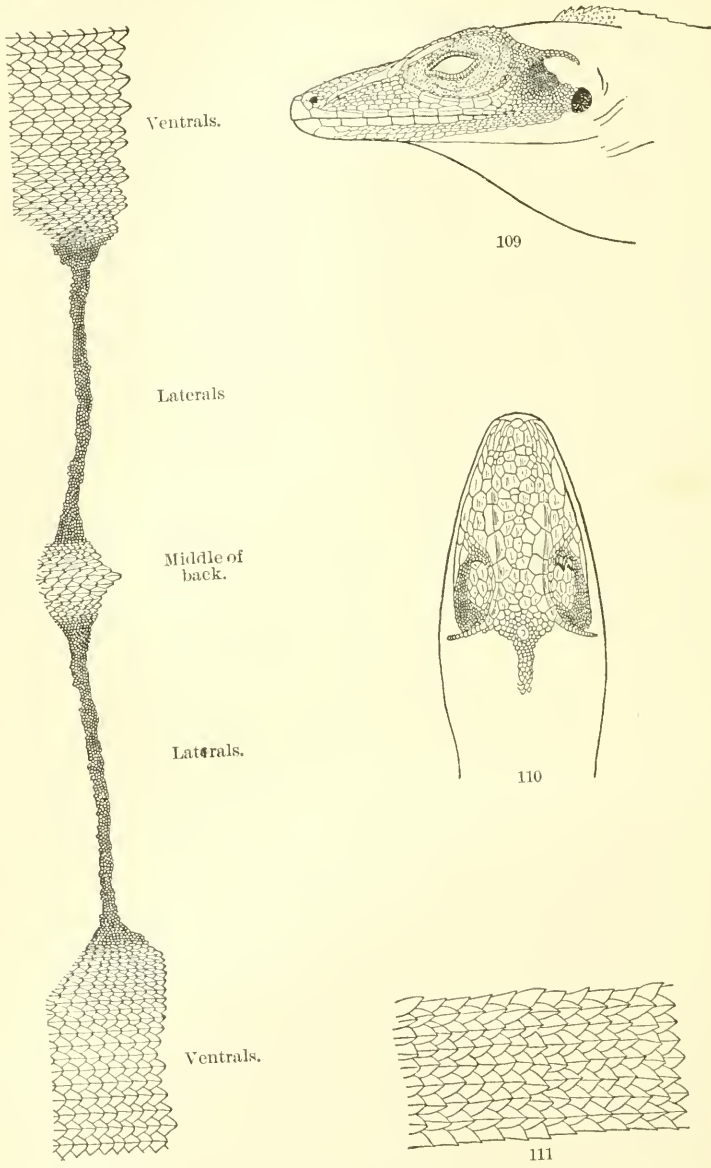
FIGS. 108-111.— ANOLIS KRUGI . 108, scales around middle of body. 5\frac{1}{2} \times natural size. 109, side of head; 110, top of head. 2\frac{3}{4} \times natural size. 111, side of tail at level of fifth verticil. 5\frac{1}{2} \times natural size. No. 26876, U.S.N.M.
