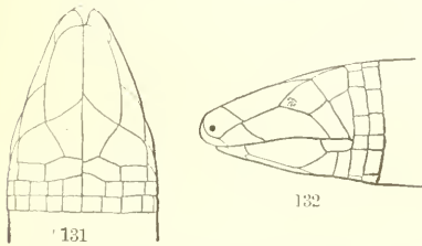
FIGS. 131-132.— AMPHISBENA CAECA . \frac{2}{3} natural size. 131, top of head; 132, side of head. No. 25510, U.S.N.M.
