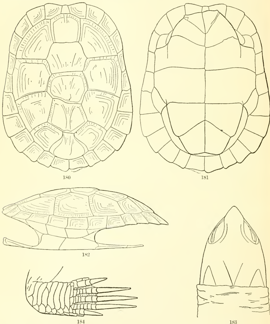
FIGS. 180-184.— PSEUDEMYDYS PALUSTRIS , young. 180, shell from above; 181, shell from below; 182, shell from side. \frac{1}{2} natural size. 183, top of head. 1\frac{1}{3} \times natural size. 184, upper side of fore foot. Natural size. No. 25643, U.S.N.M.
