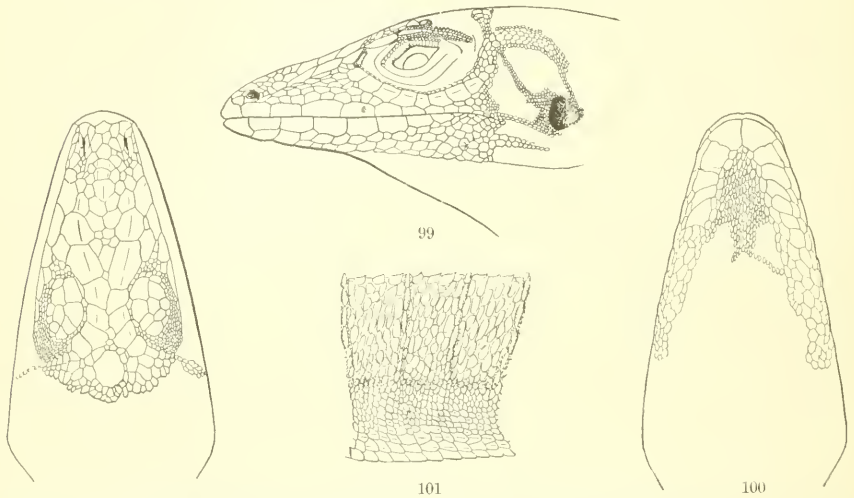
FIGS. 98-101.—ANOLIS MONENSIS. 2½ × natural size. 98, top of head; 99, side of head; 100, underside of head; 101, side of tail at level of fifth spine. No. 29387, U.S.N.M.
