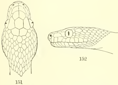
FIGS. 151-152.— EPICRATES INORNATUS , YOUNG. Natural size. 151, top of head; 152, side of head; No. 12446, U.S.N.M.
