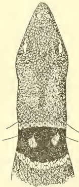
FIG. 51.—SPHLERODACTYLUS GRANDISQUAMIS. 2\frac{1}{2} \times natural size. Color pattern of head and shoulder. No. 27007, U.S.N.M.
