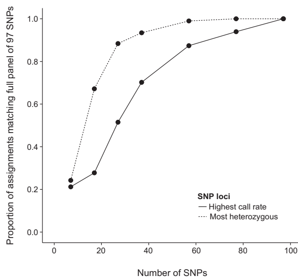
Fig. 2 Proportion of paternity assignments from decreasing numbers of single-nucleotide polymorphisms (SNPs) with the highest heterozygosity (dashed line) and highest call rates (solid line) that matched assignments of 198 black-throated blue warbler offspring using the full panel of 97 SNPs with 95% confidence.
