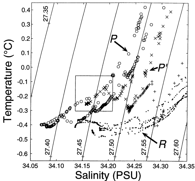
Fig. 3. Temperature-salinity diagram for the upper 200 m of the Weddell-Scotia Confluence for October-November 1993. Profiles are as shown in Fig. 2 with Sta. P (○), Sta. P' at 0900 h (×), Sta. P' at 1100 h (+), and Sta. R (●). The diagram is contoured for density at intervals of 0.05 \sigma_t . The inset box delimits water of similar T and S that was at 70–80 m at Sta. P, at the surface at Sta. P', and not found at station R.
