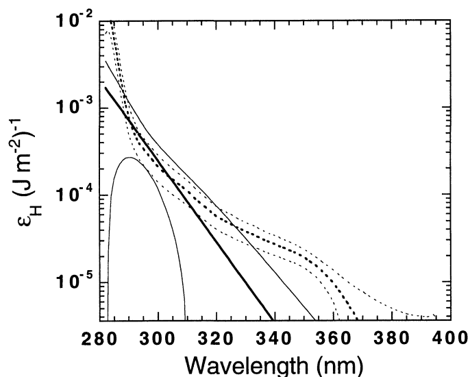
Fig. 9. BWFs for dose-dependent inhibition of photosynthesis ( \epsilon_H ) for Sta. R (2–4 November 1993) based on incubation of intact colonies (solid lines) vs. photoinhibitron measurements on homogenized samples (dotted lines). Each BWF is shown by a group of three lines—the center heavy line represents \epsilon_H(\lambda) , and the flanking lighter lines are the 95% confidence intervals. The BWF for intact colonies was estimated using data from four incubations of six spectral treatments each. The BWF follows the equation \epsilon_H(\lambda) = \exp(25.2 - 0.107\lambda) estimated by nonlinear regression ( R^2 = 0.82 ; see materials and methods). The photoinhibitron BWF is the mean for incubations conducted on 3 and 4 November (Fig. 7), with the confidence interval estimated from the standard error of the mean. The intersection of the lower confidence interval with the x -axis indicates the wavelength at which the confidence interval for \epsilon_H overlaps zero.
