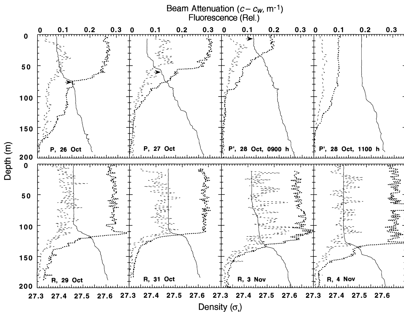
Fig. 2. Vertical profiles of density and phytoplankton parameters for stations in the Weddell-Scotia Confluence during October and November 1993: density ( \sigma_t , solid lines); beam attenuation ( c , m^{-1} , corrected for c_w , the contribution from seawater, 0.364 m^{-1} ; an indicator of particle concentration, heavy, small dashes); and active Chl fluorescence (light, large dashes). Contrasting conditions were found in the surface layer between the lighter and more stratified waters of Sta. P, which was to the south of the heavier and more strongly mixed waters of Sta. R. Sta. P' was a frontal station between the two water masses, at which conditions changed rapidly due to increased surface winds. Arrows indicate the 27.44 \sigma_t isopleth, which moved from 70 m to the surface between P and P'. At Sta. P', the contrast between an early (0900 h LT) and later (1100 h LT) morning profile shows the rapid deepening of the surface layer.
