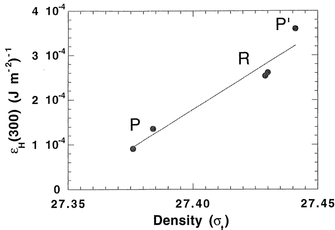
Fig. 10. Correlation between UV sensitivity and hydrography in the Weddell–Scotia Confluence. The BWF H weight at 300 nm ( \epsilon_H(300) ) is plotted as a function of sample water density ( \sigma_t ), with a line fitted by linear regression ( R^2 = 0.94 ). Annotation identifies the station sampled for each BWF. Density was not measured for the bucket sample on 30 October, so it was omitted from the analysis. In this region, higher \sigma_t in the mixed layer was associated with a greater contribution of deep water (see text and Figs. 2 and 3).
